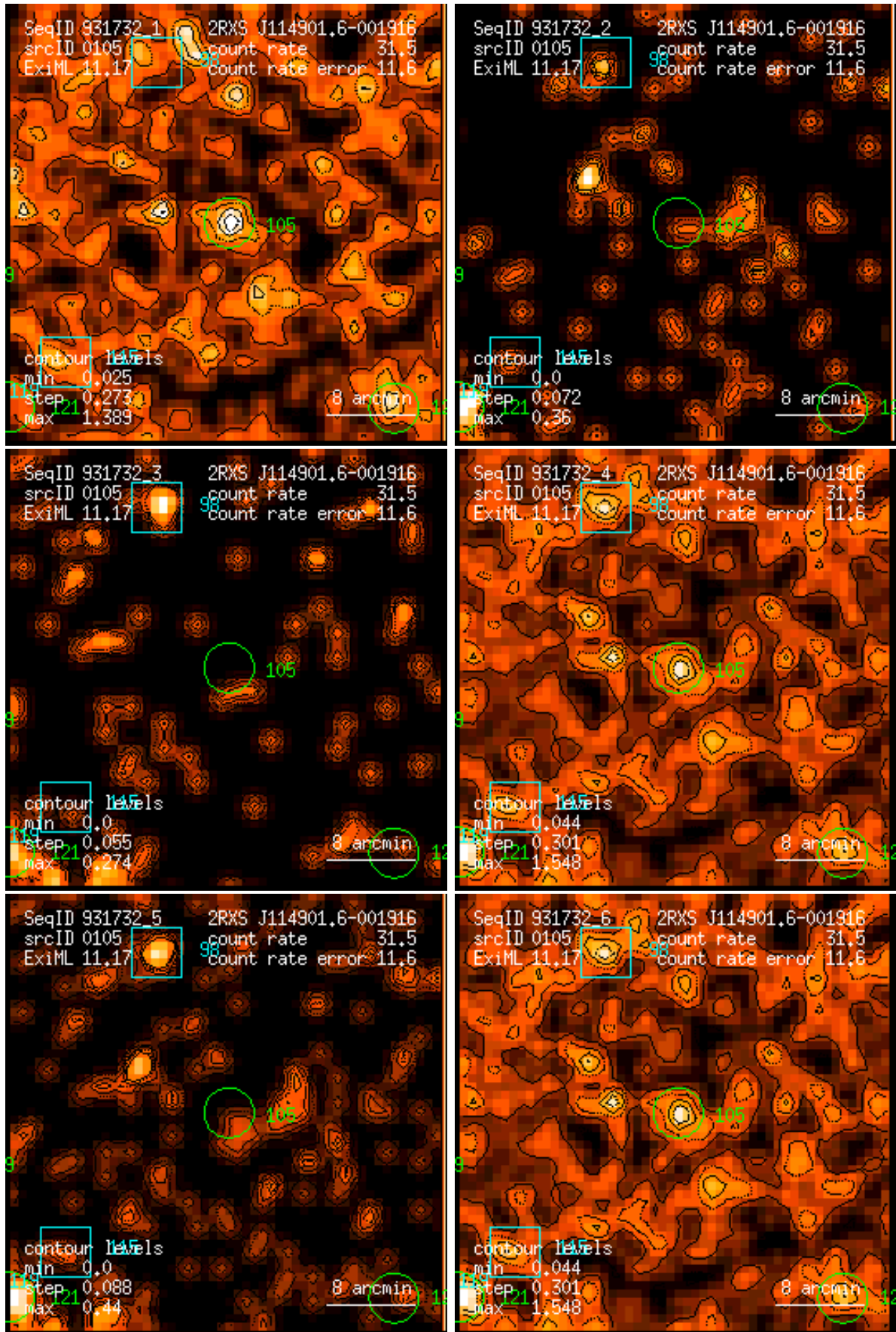
Figure 105: RASS 931732: detection 0105: band rate images, Gaussian filter: (1) PSPC channels 11 – 41, (2) 52 – 90, (3) 91 – 201, (4) 11 – 235, (5) 52 – 201, (6) 11 – 201. Broad band rates in counts/ks. Band rate contour levels in counts/ks/arcmin 2 .
