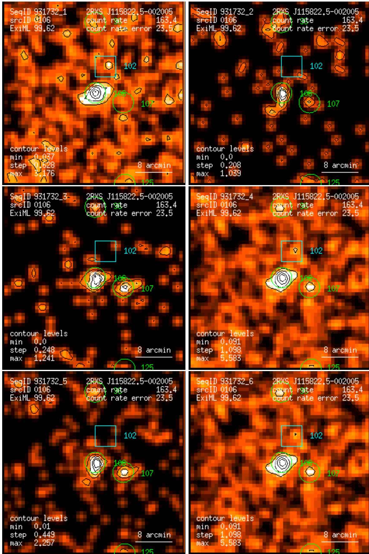
Figure 106: RASS 931732: detection 0106: band rate images, Gaussian filter: (1) PSPC channels 11 – 41, (2) 52 – 90, (3) 91 – 201, (4) 11 – 235, (5) 52 – 201, (6) 11 – 201. Broad band rates in counts/ks. Band rate contour levels in counts/ks/arcmin 2 .
