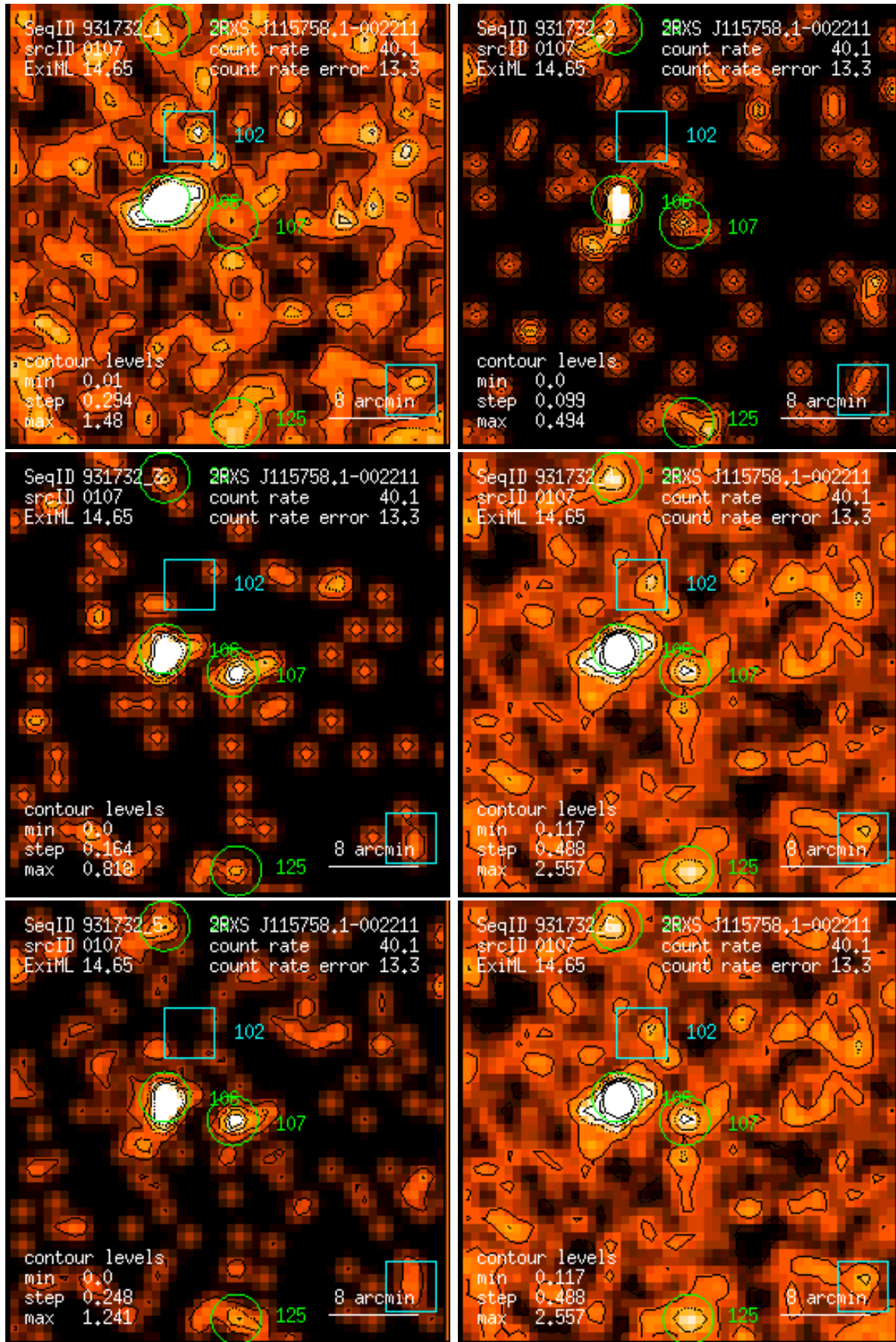
Figure 107: RASS 931732: detection 0107: band rate images, Gaussian filter: (1) PSPC channels 11 – 41, (2) 52 – 90, (3) 91 – 201, (4) 11 – 235, (5) 52 – 201, (6) 11 – 201. Broad band rates in counts/ks. Band rate contour levels in counts/ks/arcmin 2 .
