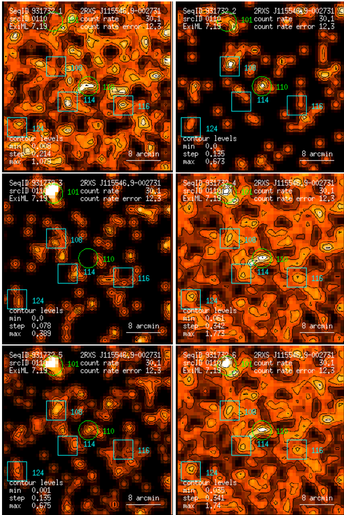
Figure 110: RASS 931732: detection 0110: band rate images, Gaussian filter: (1) PSPC channels 11 – 41, (2) 52 – 90, (3) 91 – 201, (4) 11 – 235, (5) 52 – 201, (6) 11 – 201. Broad band rates in counts/ks. Band rate contour levels in counts/ks/arcmin 2 .
