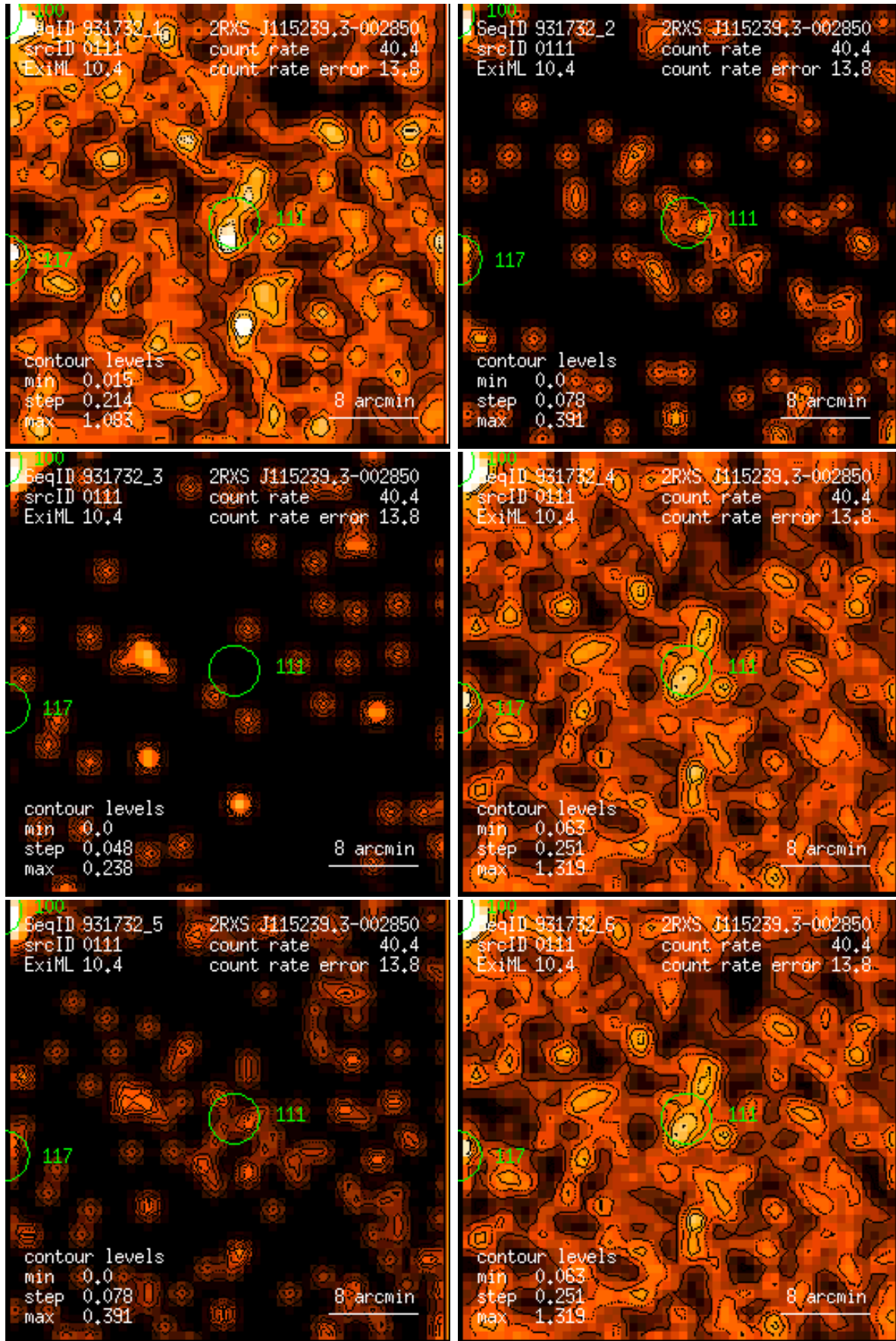
Figure 111: RASS 931732: detection 0111: band rate images, Gaussian filter: (1) PSPC channels 11 – 41, (2) 52 – 90, (3) 91 – 201, (4) 11 – 235, (5) 52 – 201, (6) 11 – 201. Broad band rates in counts/ks. Band rate contour levels in counts/ks/arcmin 2 .
