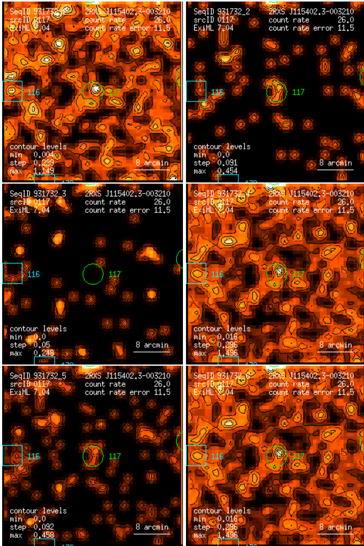
Figure 117: RASS 931732: detection 0117: band rate images, Gaussian filter: (1) PSPC channels 11 – 41, (2) 52 – 90, (3) 91 – 201, (4) 11 – 235, (5) 52 – 201, (6) 11 – 201. Broad band rates in counts/ks. Band rate contour levels in counts/ks/arcmin 2 .
