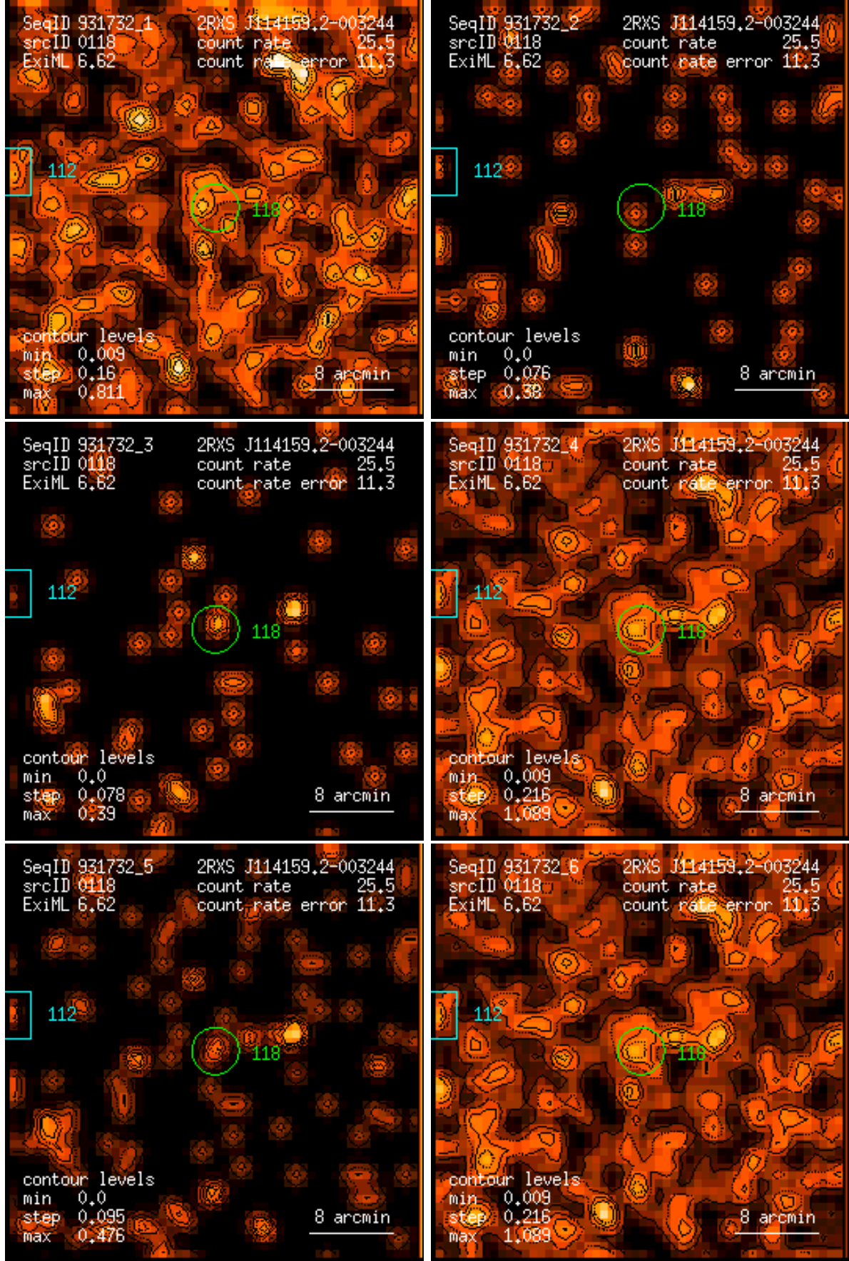
Figure 118: RASS 931732: detection 0118: band rate images, Gaussian filter: (1) PSPC channels 11 – 41, (2) 52 – 90, (3) 91 – 201, (4) 11 – 235, (5) 52 – 201, (6) 11 – 201. Broad band rates in counts/ks. Band rate contour levels in counts/ks/arcmin 2 .
