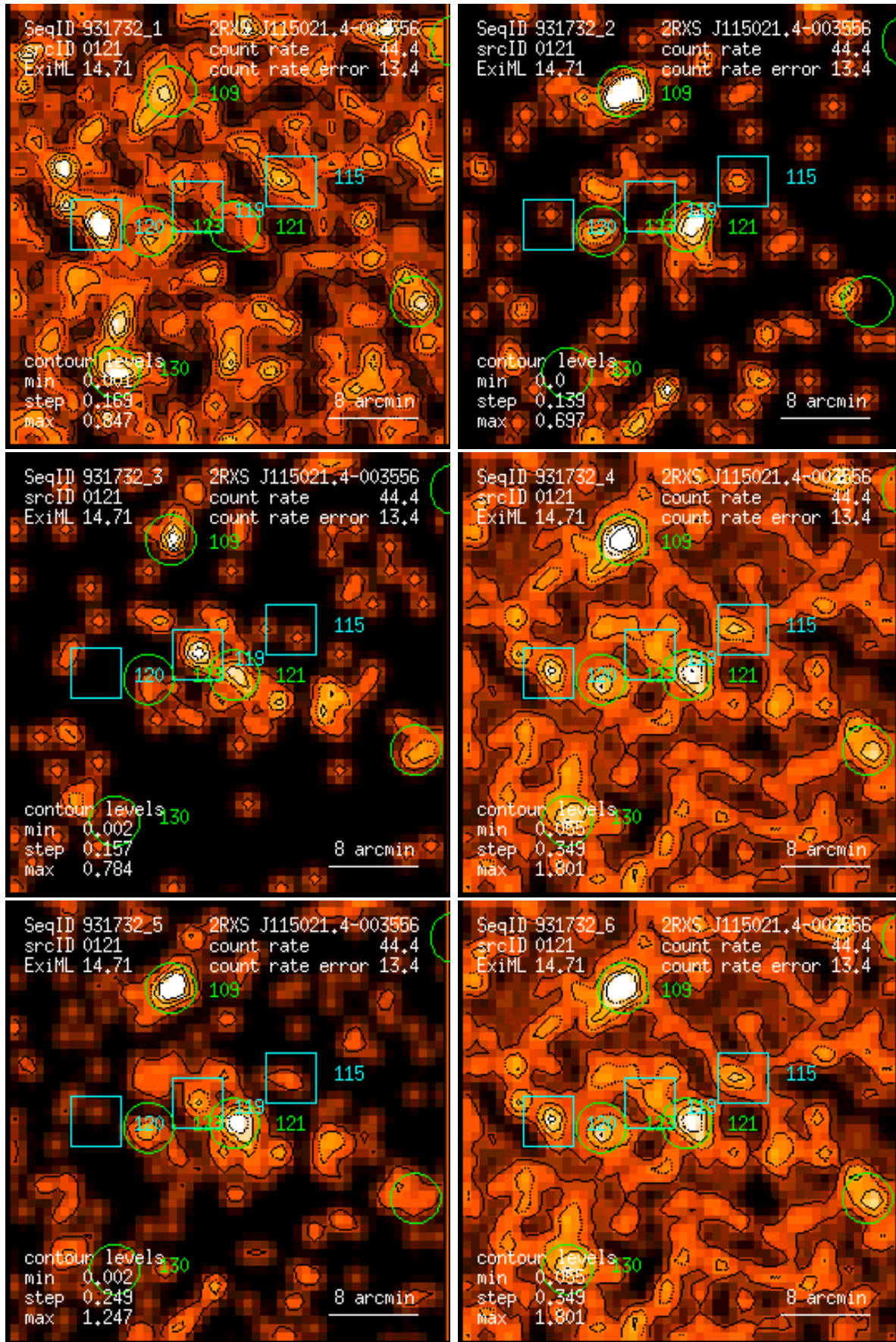
Figure 121: RASS 931732: detection 0121: band rate images, Gaussian filter: (1) PSPC channels 11 – 41, (2) 52 – 90, (3) 91 – 201, (4) 11 – 235, (5) 52 – 201, (6) 11 – 201. Broad band rates in counts/ks. Band rate contour levels in counts/ks/arcmin 2 .
