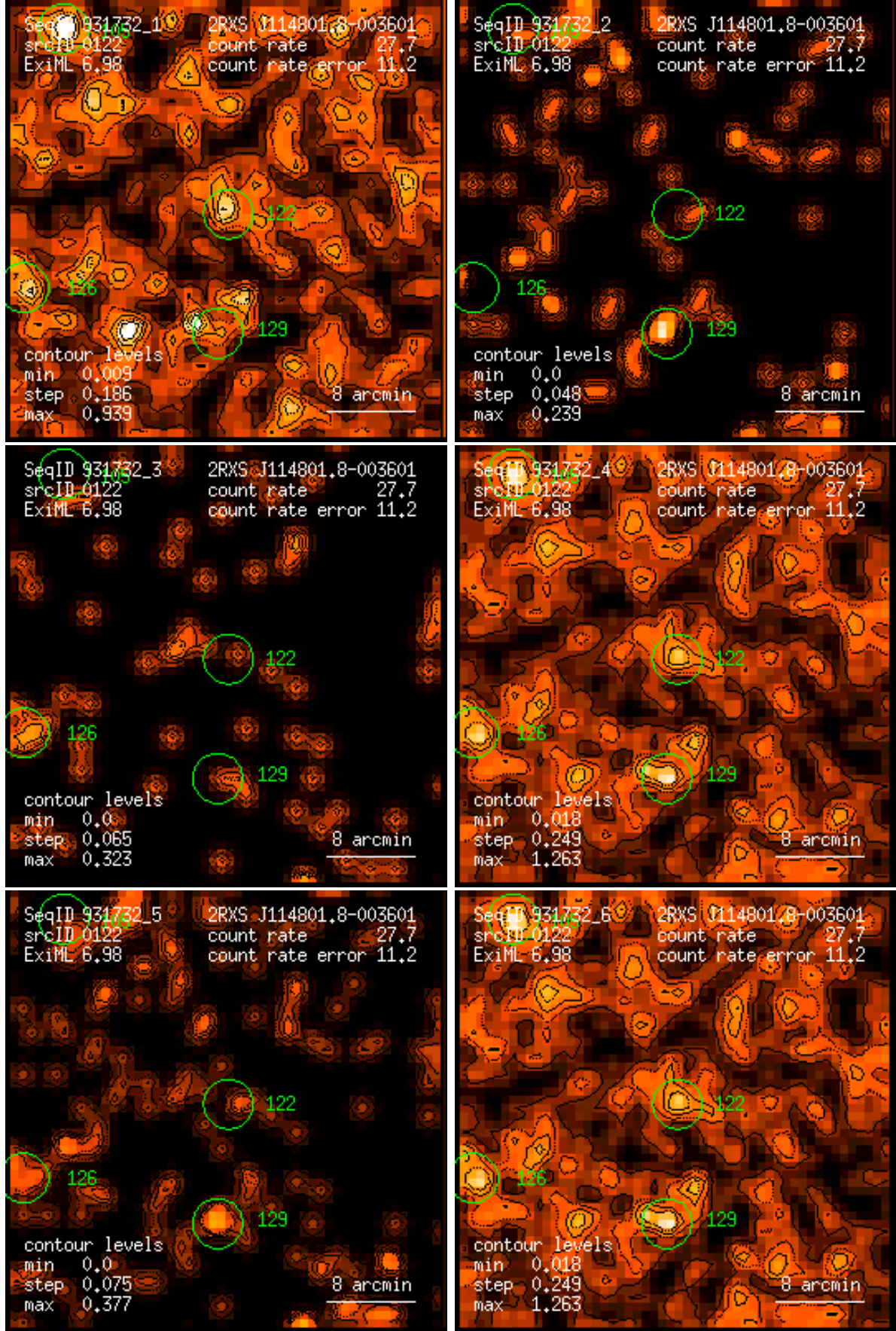
Figure 122: RASS 931732: detection 0122: band rate images, Gaussian filter: (1) PSPC channels 11 – 41, (2) 52 – 90, (3) 91 – 201, (4) 11 – 235, (5) 52 – 201, (6) 11 – 201. Broad band rates in counts/ks. Band rate contour levels in counts/ks/arcmin 2 .
