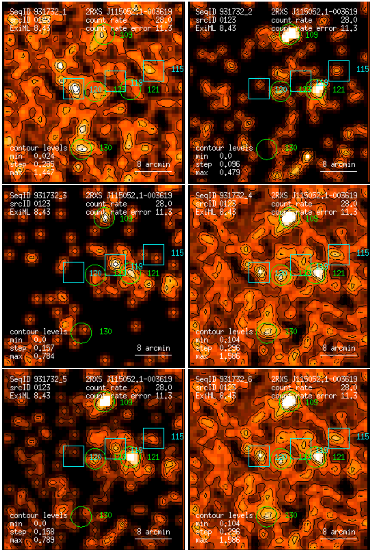
Figure 123: RASS 931732: detection 0123: band rate images, Gaussian filter: (1) PSPC channels 11 – 41, (2) 52 – 90, (3) 91 – 201, (4) 11 – 235, (5) 52 – 201, (6) 11 – 201. Broad band rates in counts/ks. Band rate contour levels in counts/ks/arcmin 2 .
