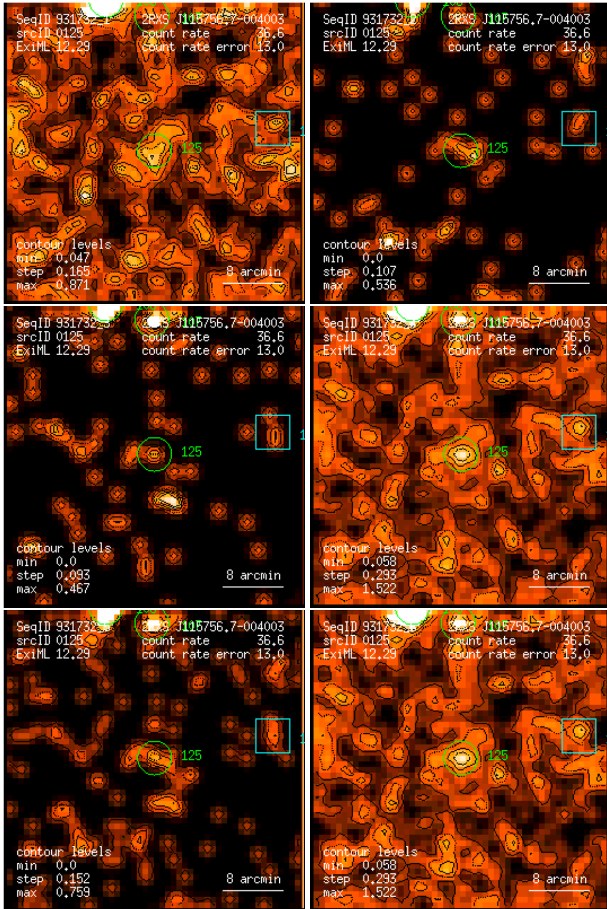
Figure 125: RASS 931732: detection 0125: band rate images, Gaussian filter: (1) PSPC channels 11 – 41, (2) 52 – 90, (3) 91 – 201, (4) 11 – 235, (5) 52 – 201, (6) 11 – 201. Broad band rates in counts/ks. Band rate contour levels in counts/ks/arcmin 2 .
