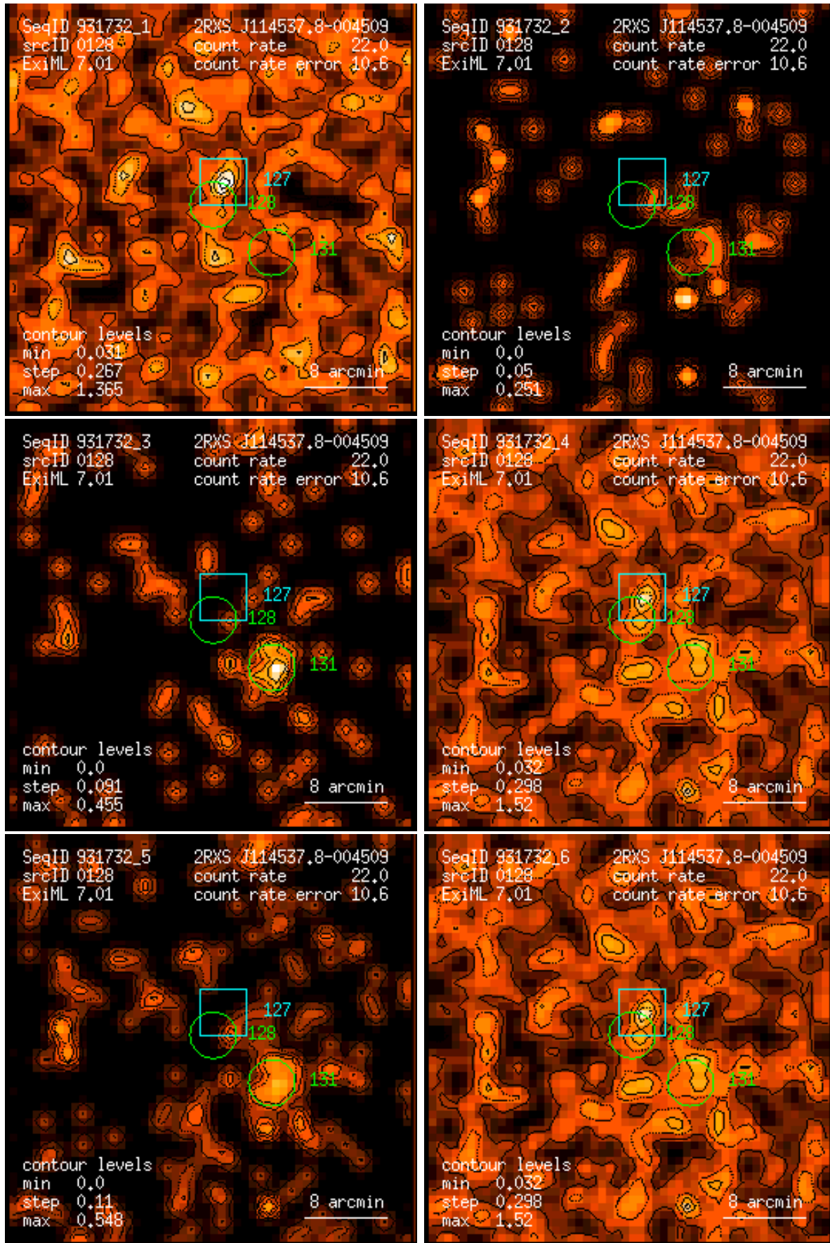
Figure 128: RASS 931732: detection 0128: band rate images, Gaussian filter: (1) PSPC channels 11 – 41, (2) 52 – 90, (3) 91 – 201, (4) 11 – 235, (5) 52 – 201, (6) 11 – 201. Broad band rates in counts/ks. Band rate contour levels in counts/ks/arcmin 2 .
