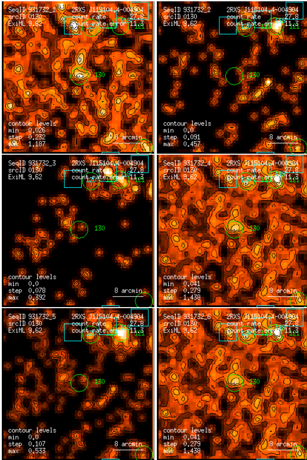
Figure 130: RASS 931732: detection 0130: band rate images, Gaussian filter: (1) PSPC channels 11 – 41, (2) 52 – 90, (3) 91 – 201, (4) 11 – 235, (5) 52 – 201, (6) 11 – 201. Broad band rates in counts/ks. Band rate contour levels in counts/ks/arcmin 2 .
