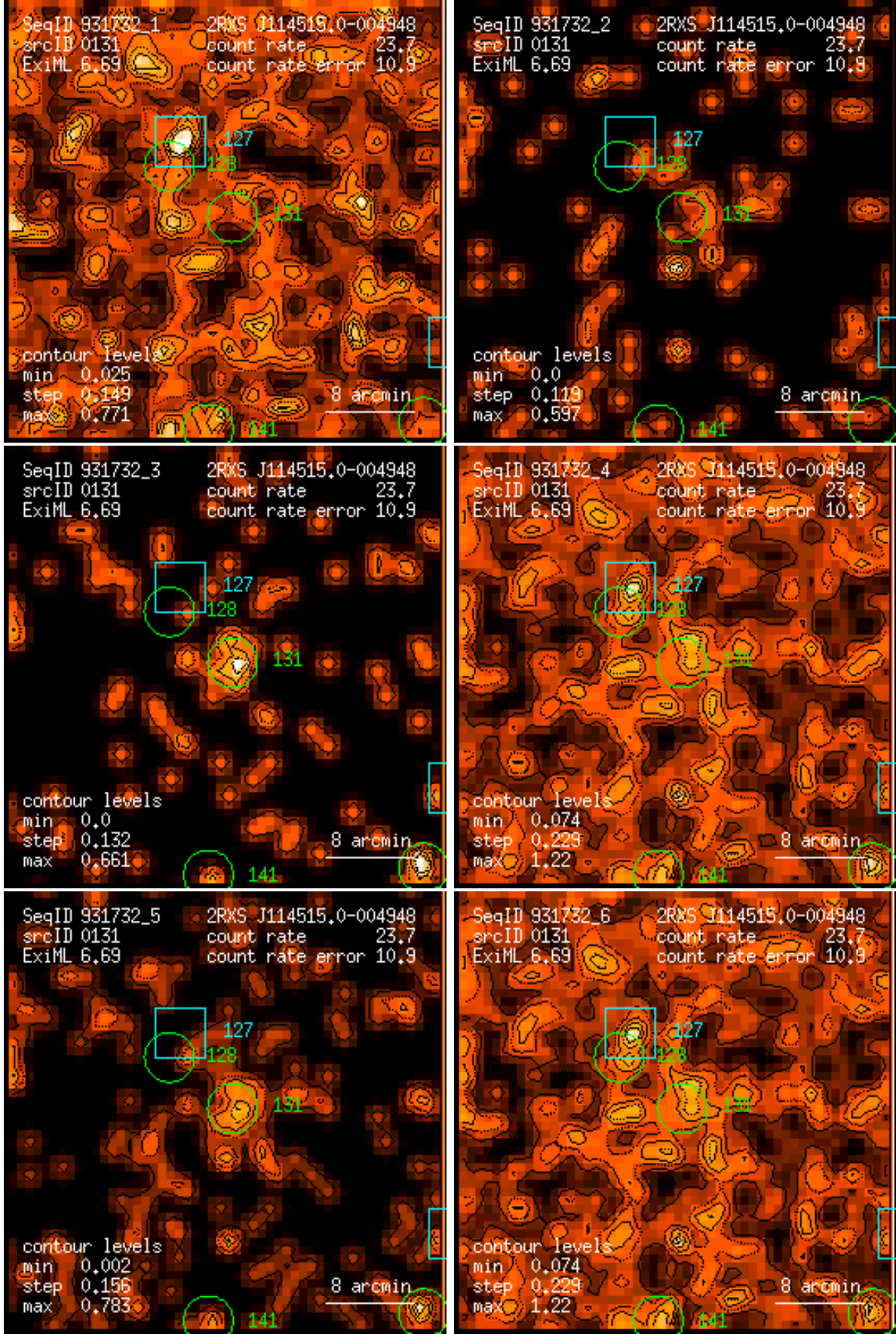
Figure 131: RASS 931732: detection 0131: band rate images, Gaussian filter: (1) PSPC channels 11 – 41, (2) 52 – 90, (3) 91 – 201, (4) 11 – 235, (5) 52 – 201, (6) 11 – 201. Broad band rates in counts/ks. Band rate contour levels in counts/ks/arcmin 2 .
