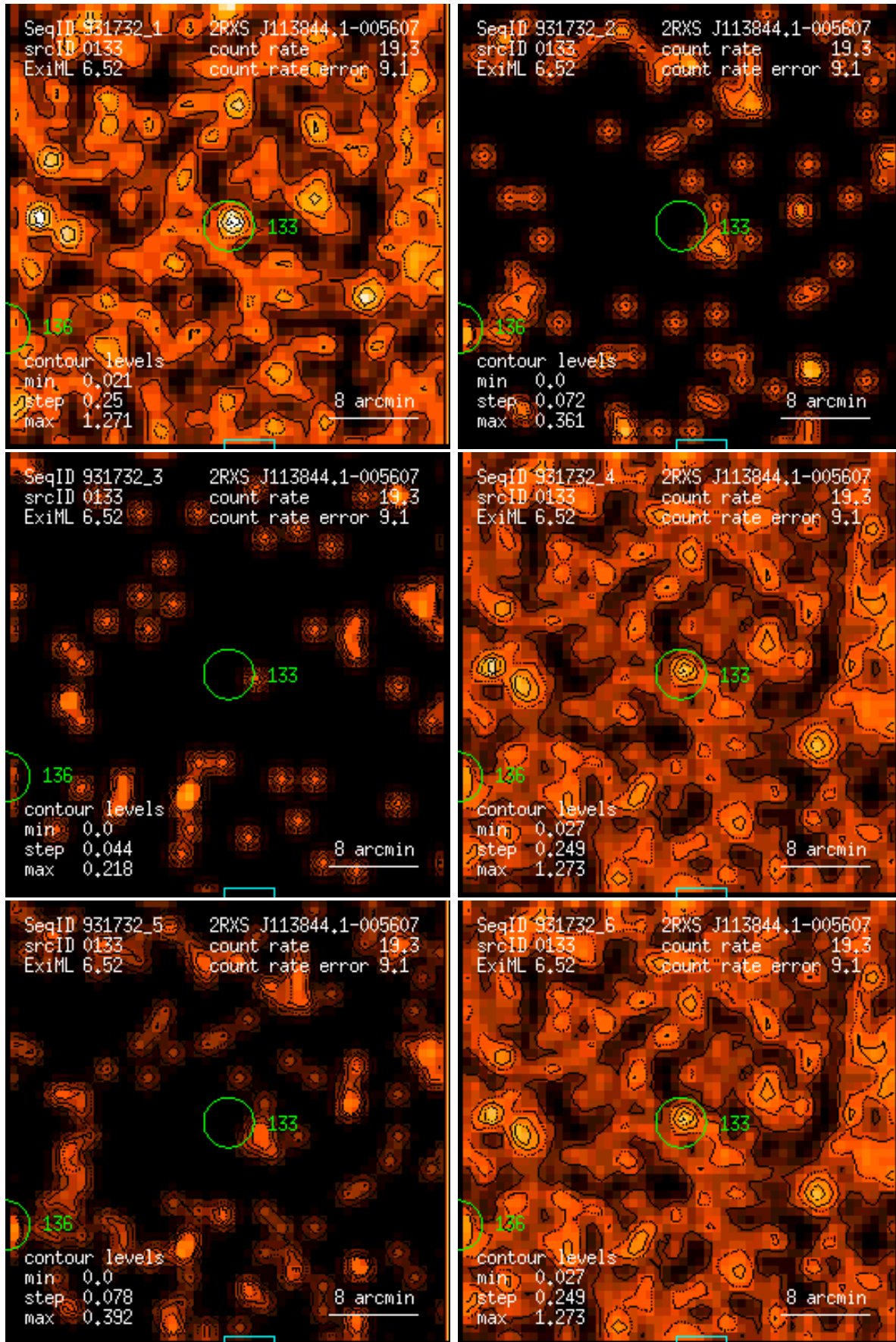
Figure 133: RASS 931732: detection 0133: band rate images, Gaussian filter: (1) PSPC channels 11 – 41, (2) 52 – 90, (3) 91 – 201, (4) 11 – 235, (5) 52 – 201, (6) 11 – 201. Broad band rates in counts/ks. Band rate contour levels in counts/ks/arcmin 2 .
