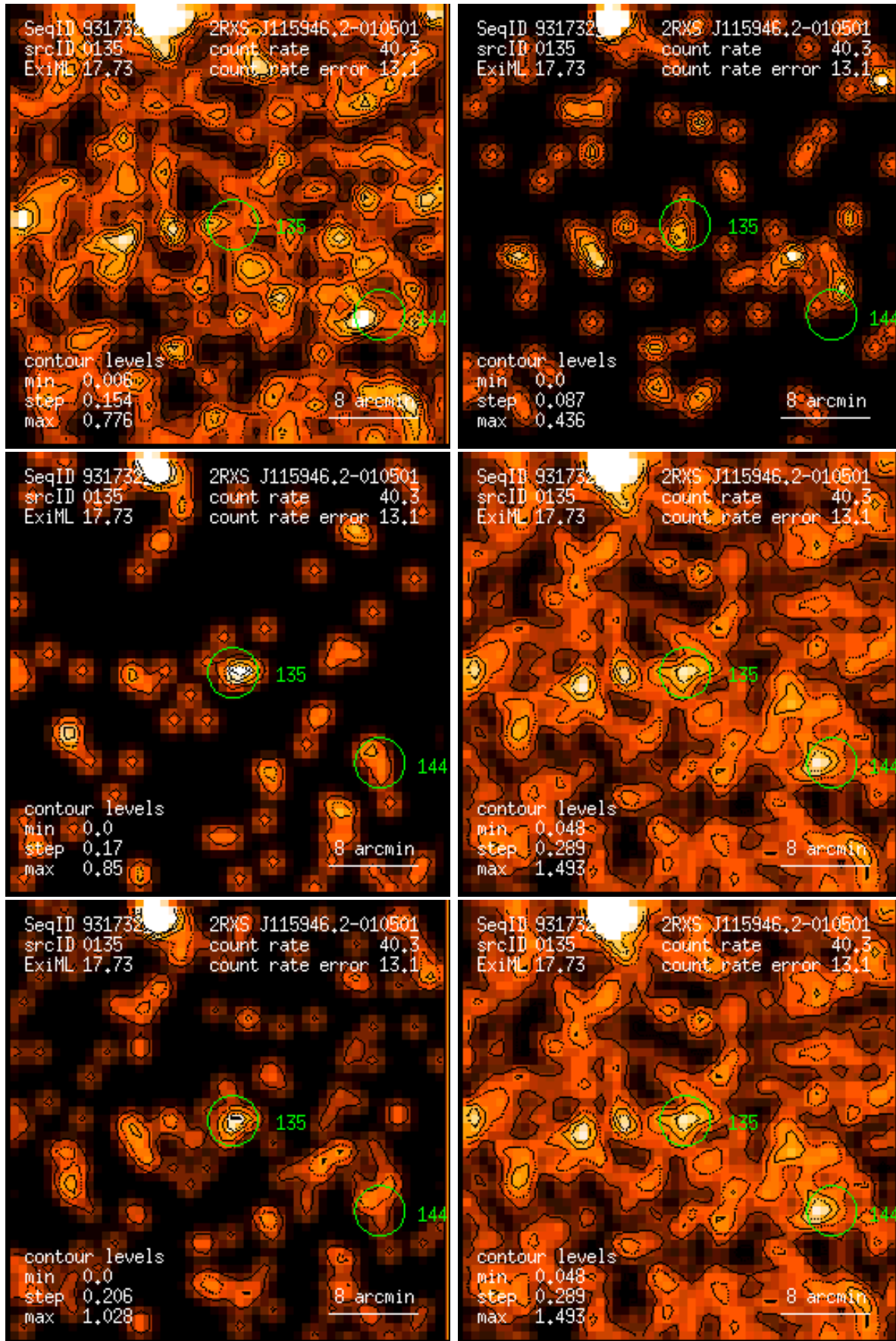
Figure 135: RASS 931732: detection 0135: band rate images, Gaussian filter: (1) PSPC channels 11 – 41, (2) 52 – 90, (3) 91 – 201, (4) 11 – 235, (5) 52 – 201, (6) 11 – 201. Broad band rates in counts/ks. Band rate contour levels in counts/ks/arcmin 2 .
