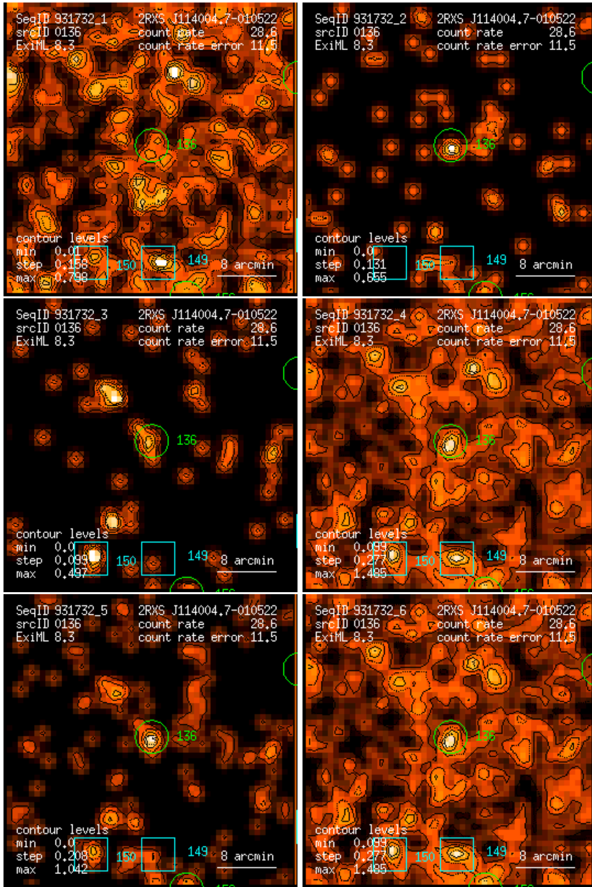
Figure 136: RASS 931732: detection 0136: band rate images, Gaussian filter: (1) PSPC channels 11 – 41, (2) 52 – 90, (3) 91 – 201, (4) 11 – 235, (5) 52 – 201, (6) 11 – 201. Broad band rates in counts/ks. Band rate contour levels in counts/ks/arcmin 2 .
