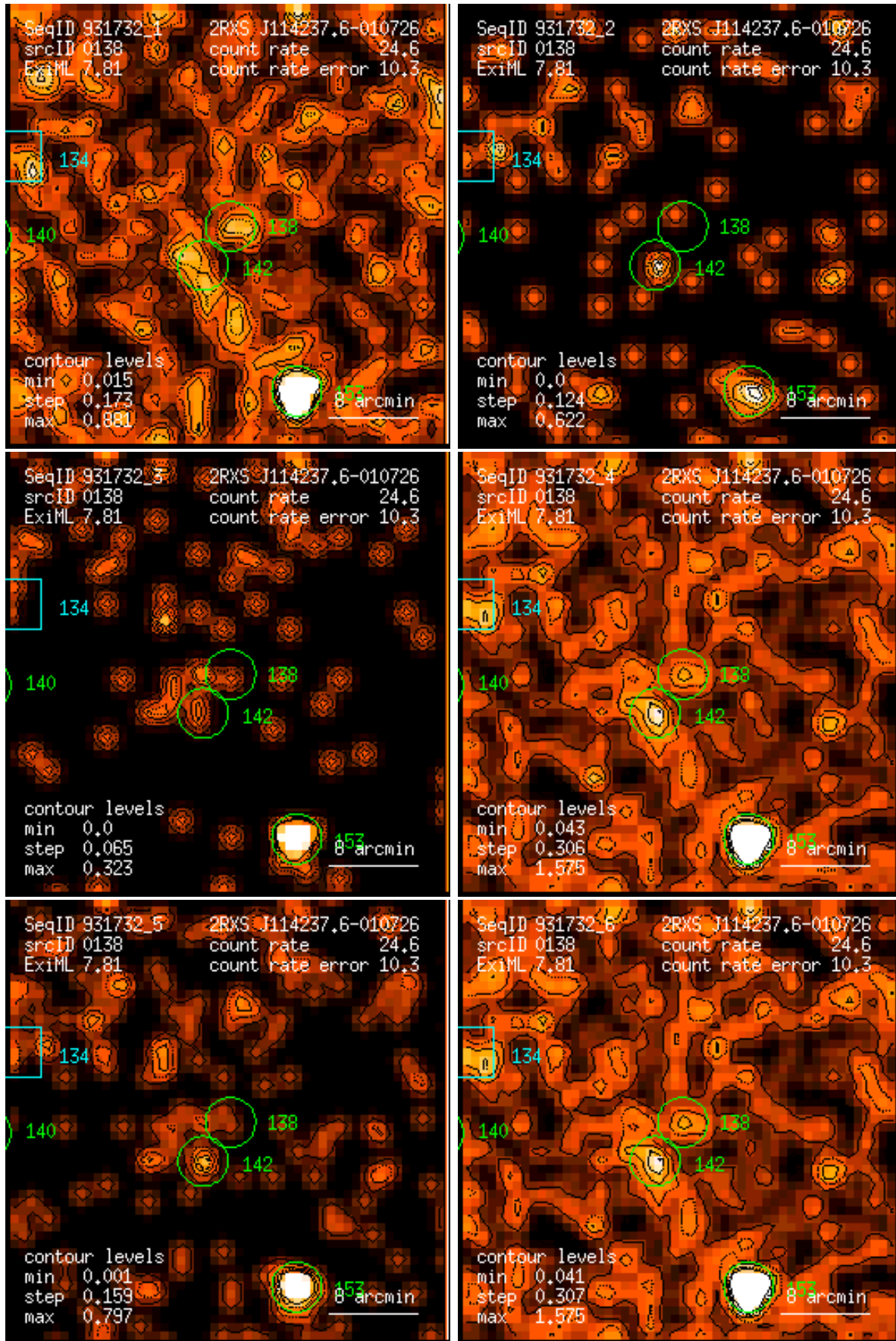
Figure 138: RASS 931732: detection 0138: band rate images, Gaussian filter: (1) PSPC channels 11 – 41, (2) 52 – 90, (3) 91 – 201, (4) 11 – 235, (5) 52 – 201, (6) 11 – 201. Broad band rates in counts/ks. Band rate contour levels in counts/ks/arcmin 2 .
