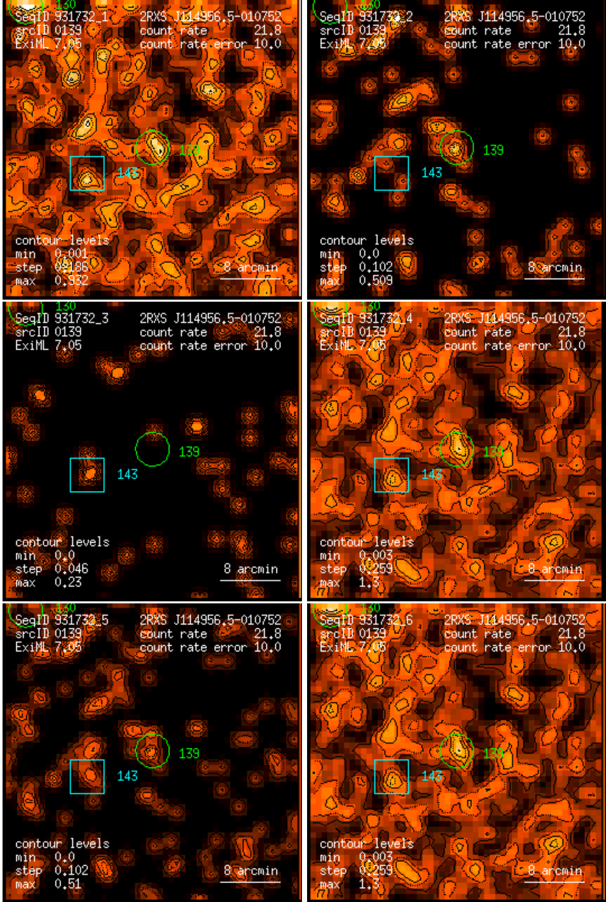
Figure 139: RASS 931732: detection 0139: band rate images, Gaussian filter: (1) PSPC channels 11 – 41, (2) 52 – 90, (3) 91 – 201, (4) 11 – 235, (5) 52 – 201, (6) 11 – 201. Broad band rates in counts/ks. Band rate contour levels in counts/ks/arcmin 2 .
