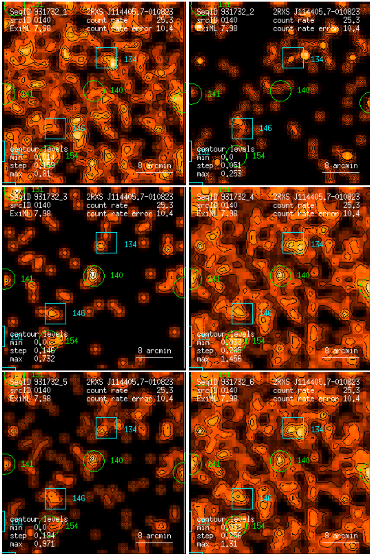
Figure 140: RASS 931732: detection 0140: band rate images, Gaussian filter: (1) PSPC channels 11 – 41, (2) 52 – 90, (3) 91 – 201, (4) 11 – 235, (5) 52 – 201, (6) 11 – 201. Broad band rates in counts/ks. Band rate contour levels in counts/ks/arcmin 2 .
