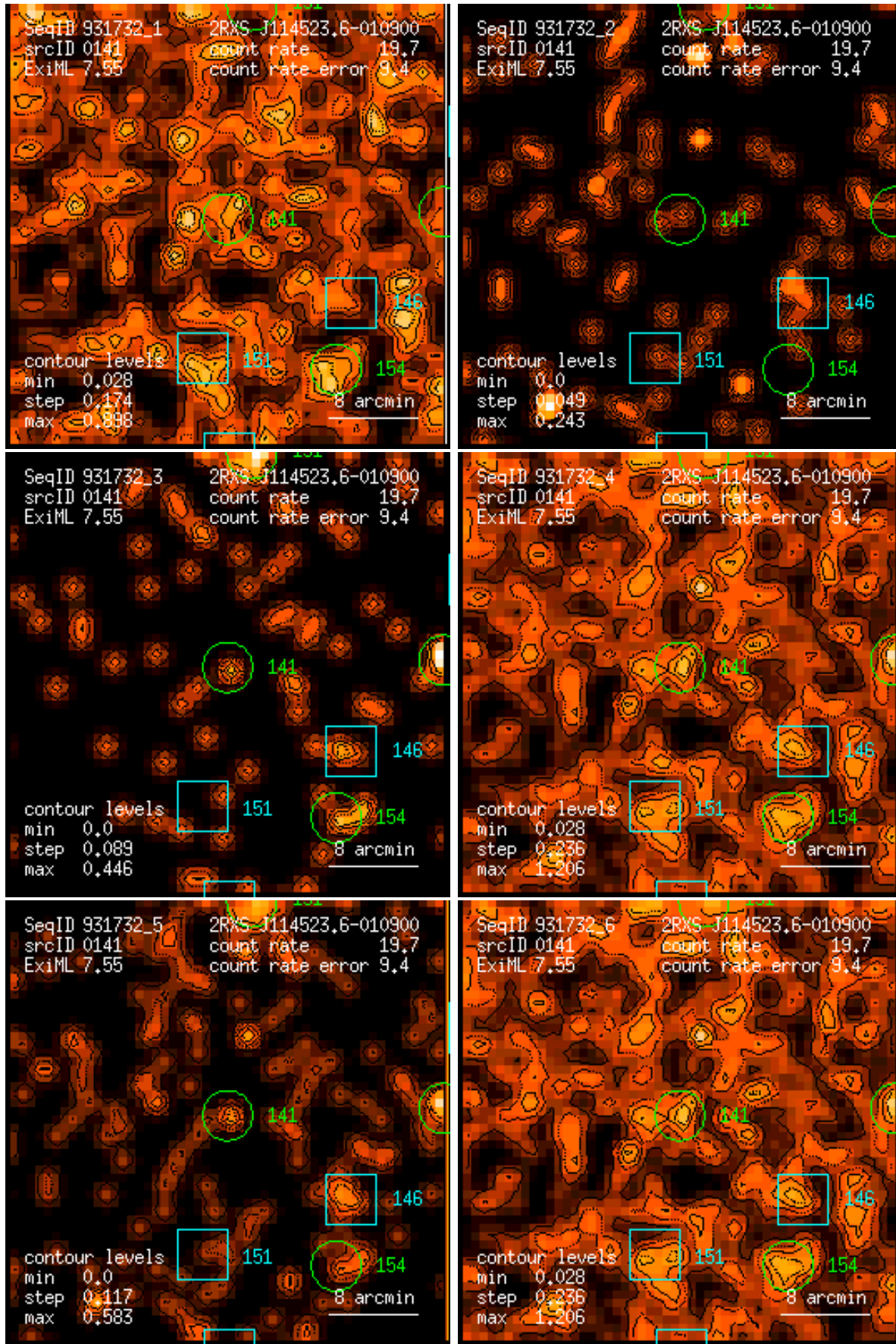
Figure 141: RASS 931732: detection 0141: band rate images, Gaussian filter: (1) PSPC channels 11 – 41, (2) 52 – 90, (3) 91 – 201, (4) 11 – 235, (5) 52 – 201, (6) 11 – 201. Broad band rates in counts/ks. Band rate contour levels in counts/ks/arcmin 2 .
