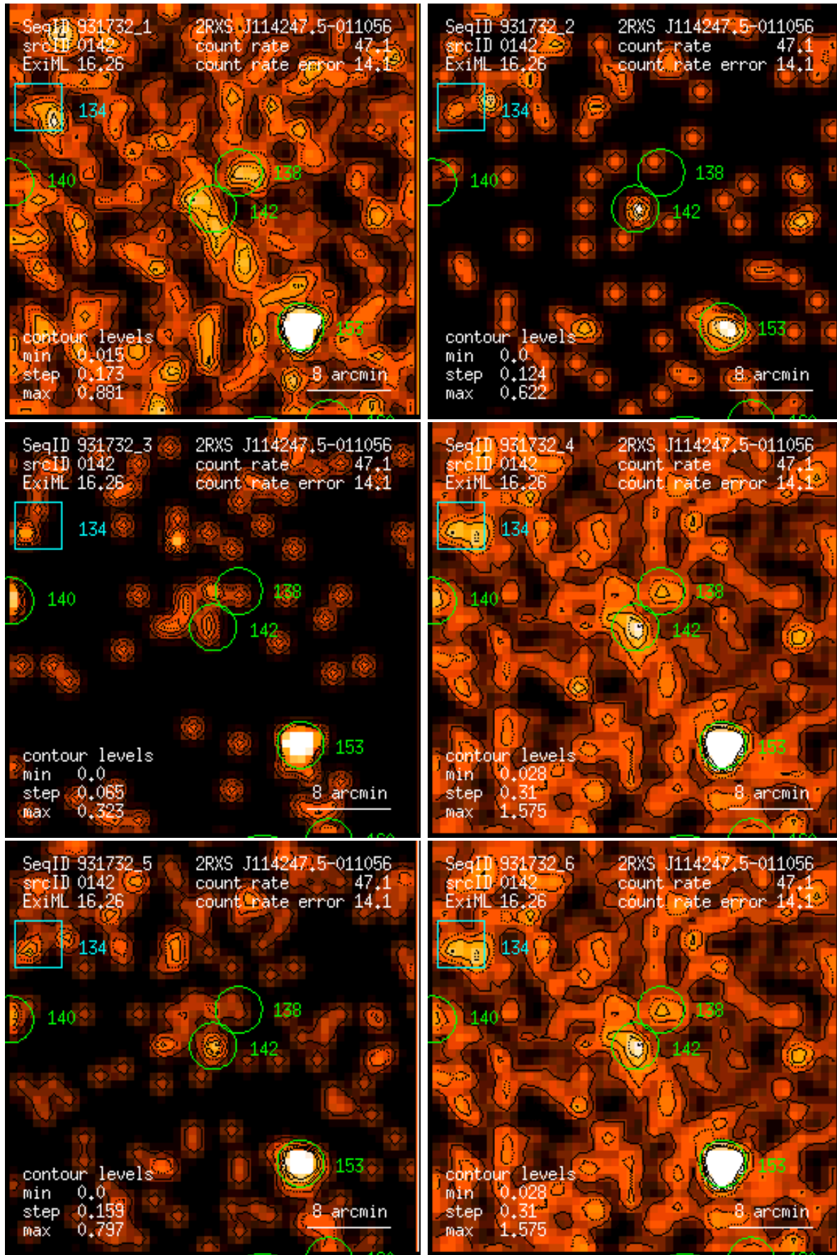
Figure 142: RASS 931732: detection 0142: band rate images, Gaussian filter: (1) PSPC channels 11 – 41, (2) 52 – 90, (3) 91 – 201, (4) 11 – 235, (5) 52 – 201, (6) 11 – 201. Broad band rates in counts/ks. Band rate contour levels in counts/ks/arcmin 2 .
