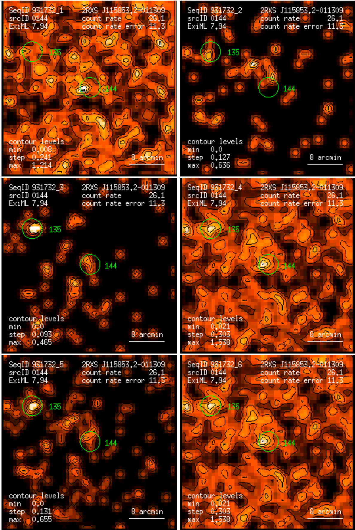
Figure 144: RASS 931732: detection 0144: band rate images, Gaussian filter: (1) PSPC channels 11 – 41, (2) 52 – 90, (3) 91 – 201, (4) 11 – 235, (5) 52 – 201, (6) 11 – 201. Broad band rates in counts/ks. Band rate contour levels in counts/ks/arcmin 2 .
