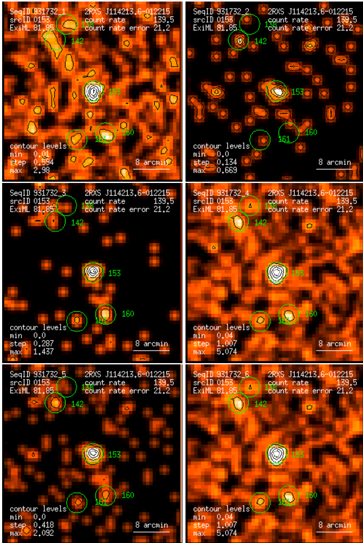
Figure 153: RASS 931732: detection 0153: band rate images, Gaussian filter: (1) PSPC channels 11 – 41, (2) 52 – 90, (3) 91 – 201, (4) 11 – 235, (5) 52 – 201, (6) 11 – 201. Broad band rates in counts/ks. Band rate contour levels in counts/ks/arcmin 2 .
