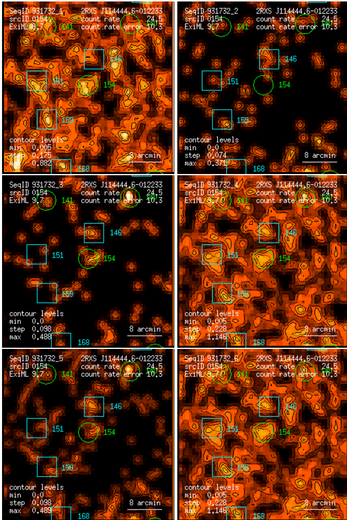
Figure 154: RASS 931732: detection 0154: band rate images, Gaussian filter: (1) PSPC channels 11 – 41, (2) 52 – 90, (3) 91 – 201, (4) 11 – 235, (5) 52 – 201, (6) 11 – 201. Broad band rates in counts/ks. Band rate contour levels in counts/ks/arcmin 2 .
