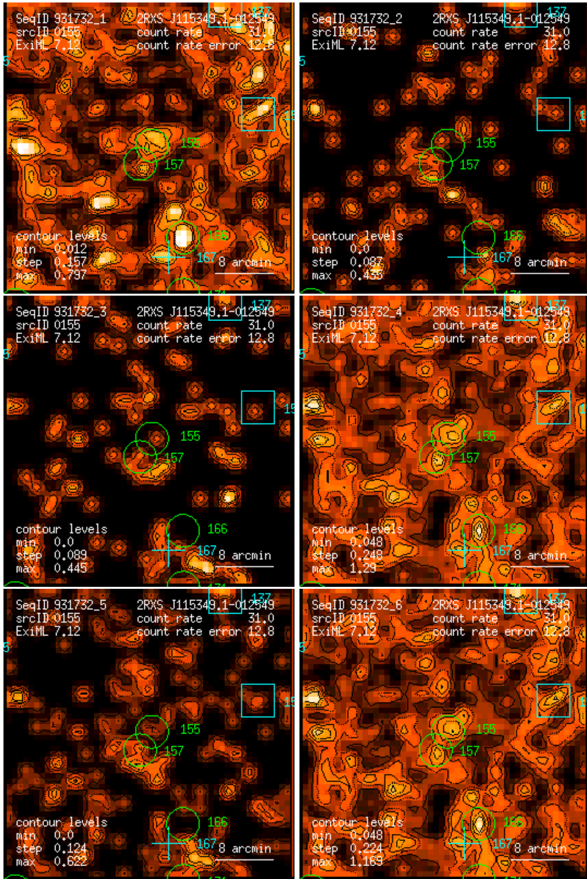
Figure 155: RASS 931732: detection 0155: band rate images, Gaussian filter: (1) PSPC channels 11 – 41, (2) 52 – 90, (3) 91 – 201, (4) 11 – 235, (5) 52 – 201, (6) 11 – 201. Broad band rates in counts/ks. Band rate contour levels in counts/ks/arcmin 2 .
