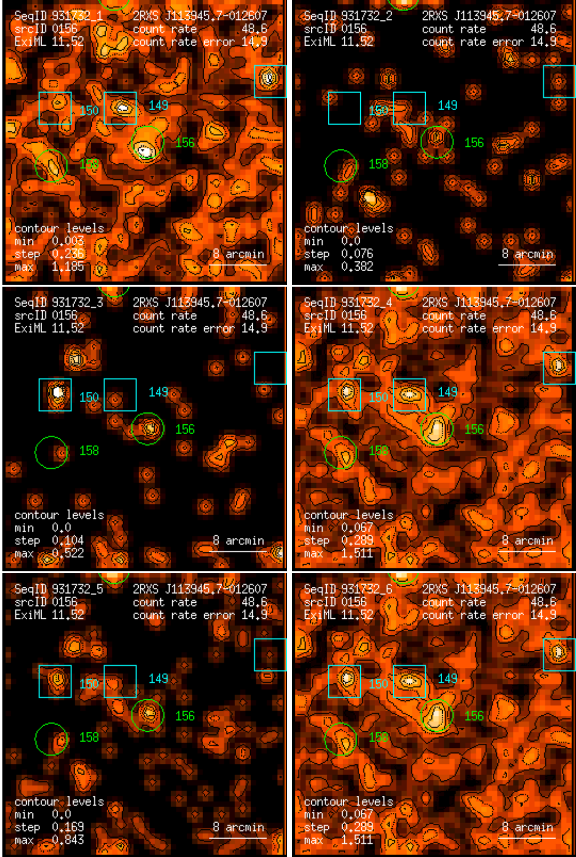
Figure 156: RASS 931732: detection 0156: band rate images, Gaussian filter: (1) PSPC channels 11 – 41, (2) 52 – 90, (3) 91 – 201, (4) 11 – 235, (5) 52 – 201, (6) 11 – 201. Broad band rates in counts/ks. Band rate contour levels in counts/ks/arcmin 2 .
