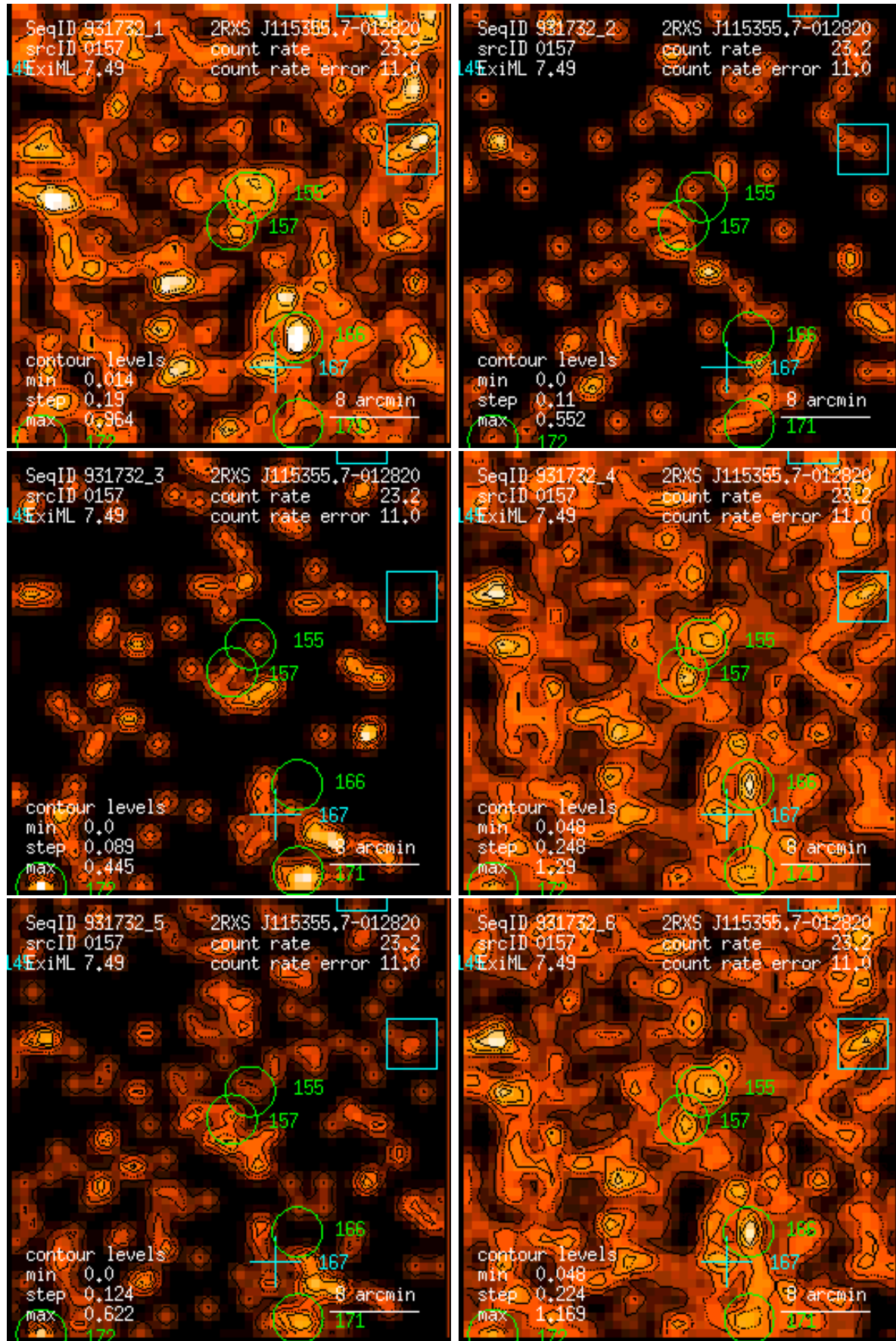
Figure 157: RASS 931732: detection 0157: band rate images, Gaussian filter: (1) PSPC channels 11 – 41, (2) 52 – 90, (3) 91 – 201, (4) 11 – 235, (5) 52 – 201, (6) 11 – 201. Broad band rates in counts/ks. Band rate contour levels in counts/ks/arcmin 2 .
