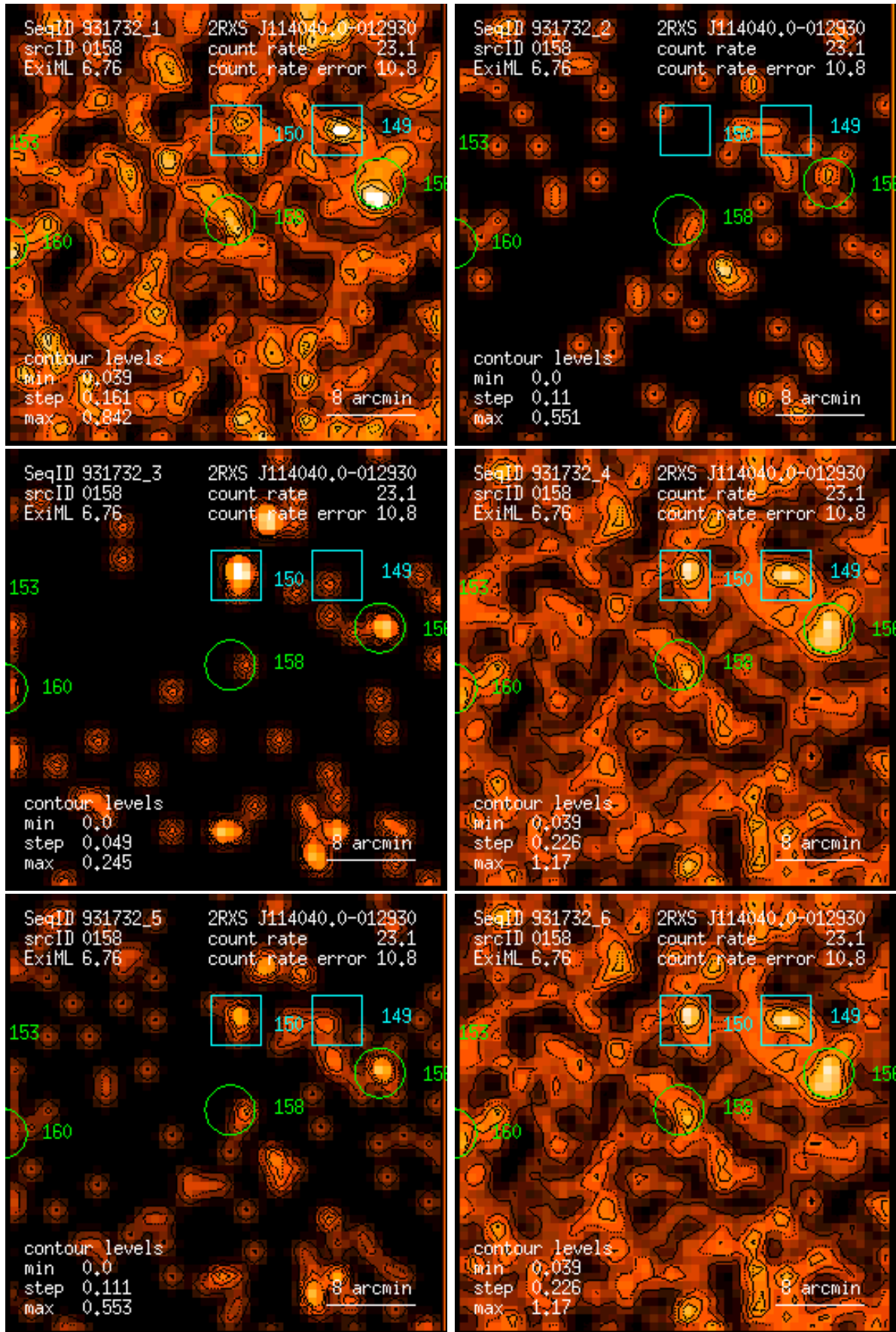
Figure 158: RASS 931732: detection 0158: band rate images, Gaussian filter: (1) PSPC channels 11 – 41, (2) 52 – 90, (3) 91 – 201, (4) 11 – 235, (5) 52 – 201, (6) 11 – 201. Broad band rates in counts/ks. Band rate contour levels in counts/ks/arcmin 2 .
