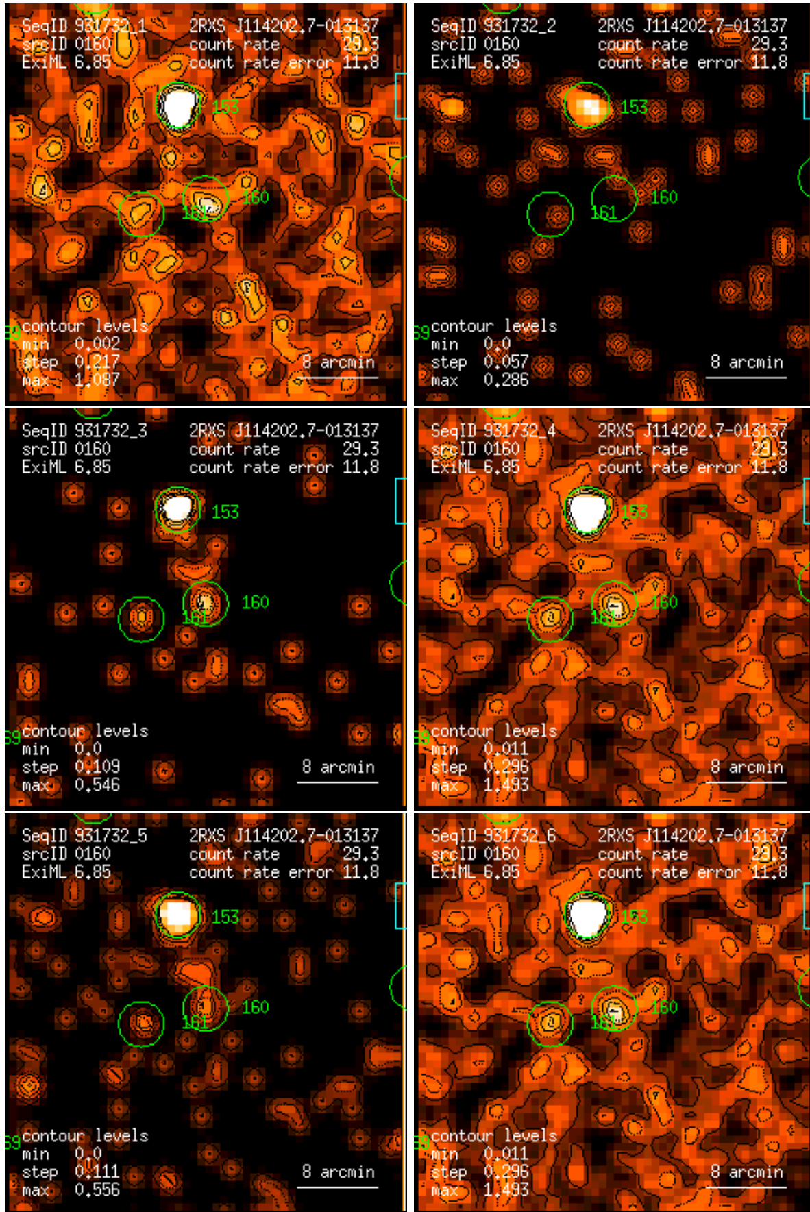
Figure 160: RASS 931732: detection 0160: band rate images, Gaussian filter: (1) PSPC channels 11 – 41, (2) 52 – 90, (3) 91 – 201, (4) 11 – 235, (5) 52 – 201, (6) 11 – 201. Broad band rates in counts/ks. Band rate contour levels in counts/ks/arcmin 2 .
