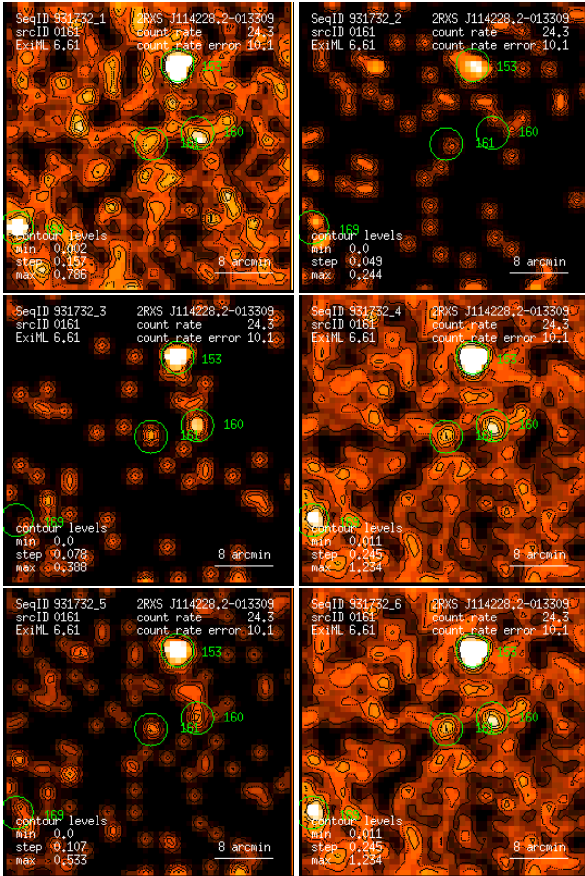
Figure 161: RASS 931732: detection 0161: band rate images, Gaussian filter: (1) PSPC channels 11 – 41, (2) 52 – 90, (3) 91 – 201, (4) 11 – 235, (5) 52 – 201, (6) 11 – 201. Broad band rates in counts/ks. Band rate contour levels in counts/ks/arcmin 2 .
