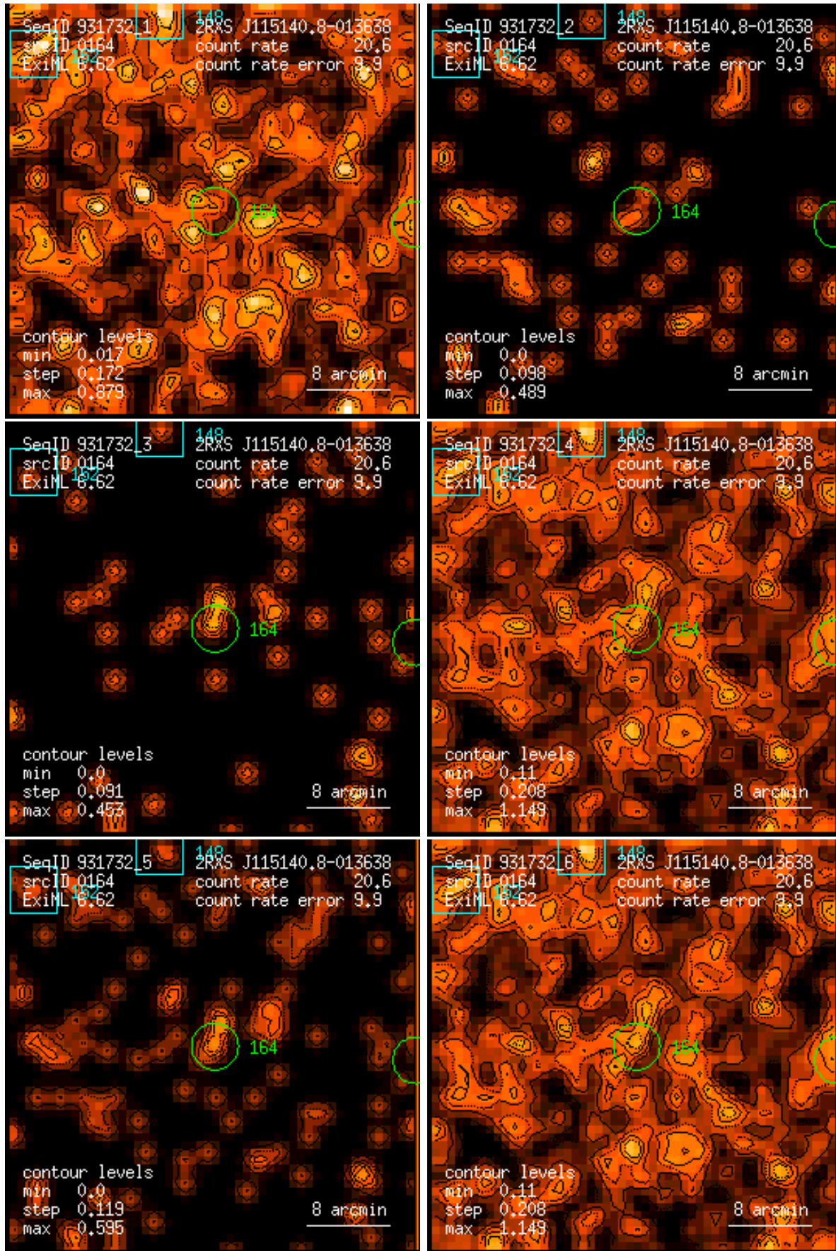
Figure 164: RASS 931732: detection 0164: band rate images, Gaussian filter: (1) PSPC channels 11 – 41, (2) 52 – 90, (3) 91 – 201, (4) 11 – 235, (5) 52 – 201, (6) 11 – 201. Broad band rates in counts/ks. Band rate contour levels in counts/ks/arcmin 2 .
