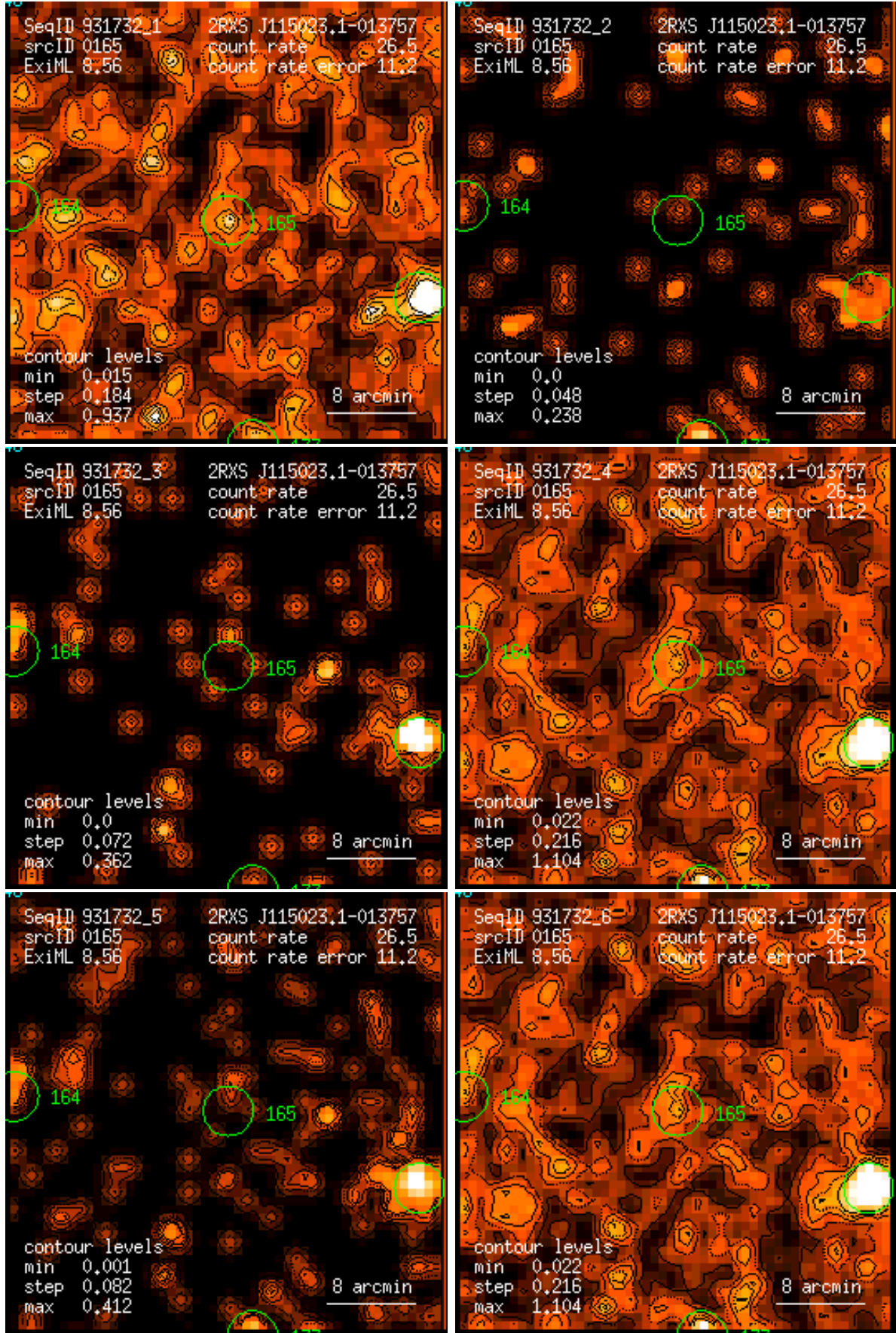
Figure 165: RASS 931732: detection 0165: band rate images, Gaussian filter: (1) PSPC channels 11 – 41, (2) 52 – 90, (3) 91 – 201, (4) 11 – 235, (5) 52 – 201, (6) 11 – 201. Broad band rates in counts/ks. Band rate contour levels in counts/ks/arcmin 2 .
