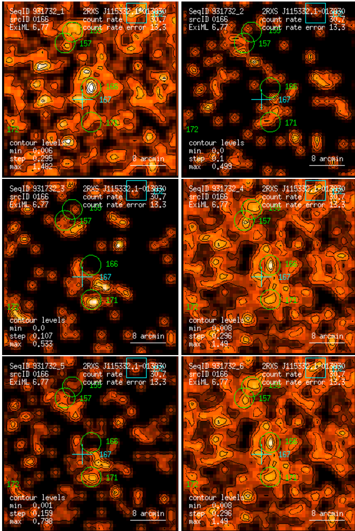
Figure 166: RASS 931732: detection 0166: band rate images, Gaussian filter: (1) PSPC channels 11 – 41, (2) 52 – 90, (3) 91 – 201, (4) 11 – 235, (5) 52 – 201, (6) 11 – 201. Broad band rates in counts/ks. Band rate contour levels in counts/ks/arcmin 2 .
