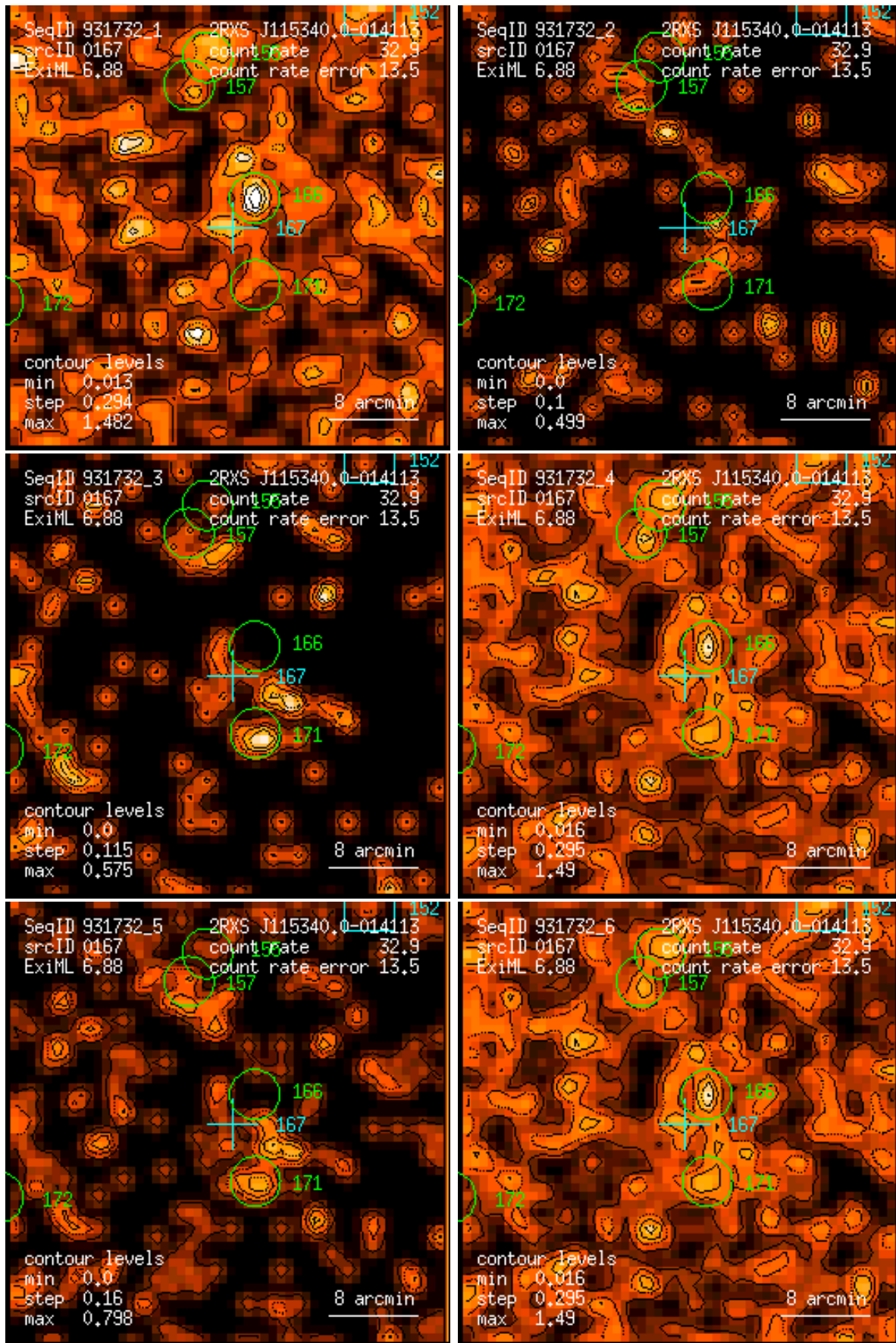
Figure 167: RASS 931732: detection 0167: band rate images, Gaussian filter: (1) PSPC channels 11 – 41, (2) 52 – 90, (3) 91 – 201, (4) 11 – 235, (5) 52 – 201, (6) 11 – 201. Broad band rates in counts/ks. Band rate contour levels in counts/ks/arcmin 2 .
