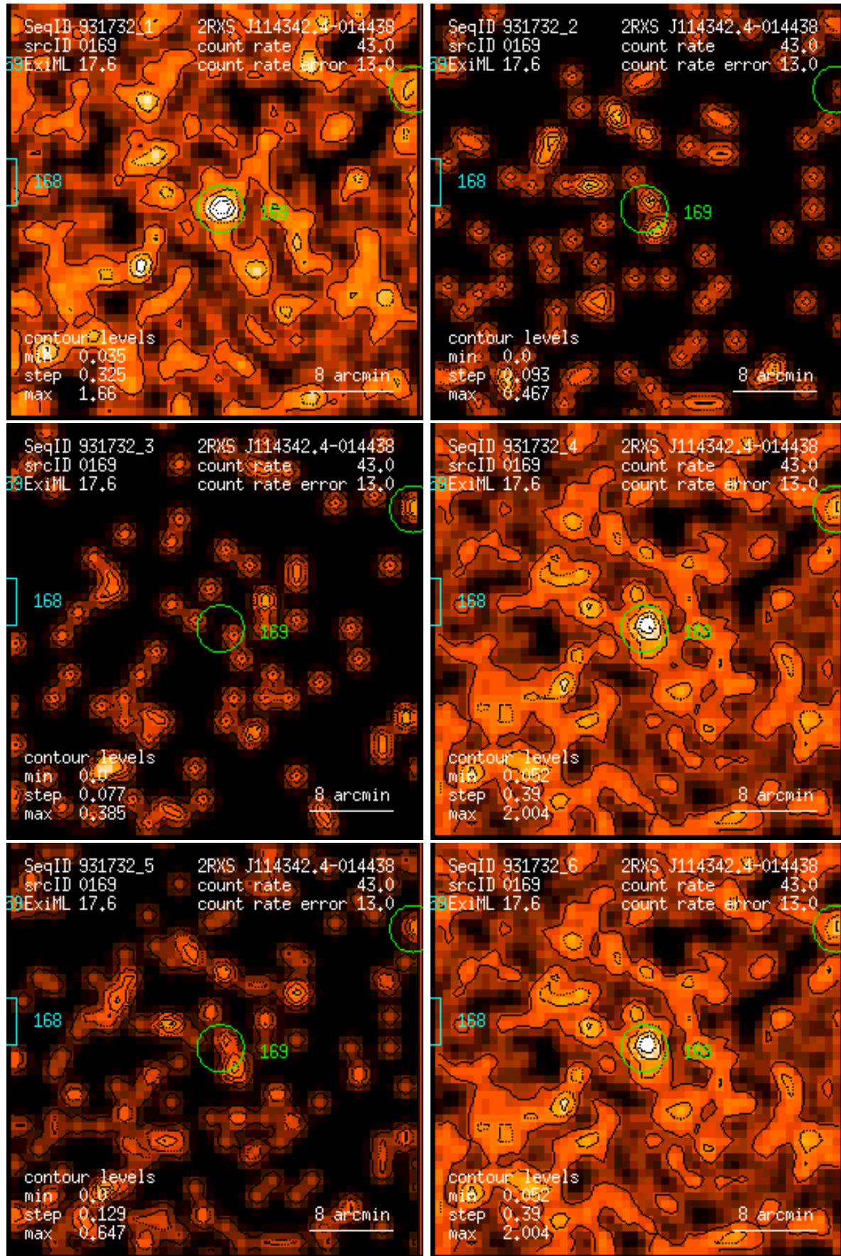
Figure 169: RASS 931732: detection 0169: band rate images, Gaussian filter: (1) PSPC channels 11 – 41, (2) 52 – 90, (3) 91 – 201, (4) 11 – 235, (5) 52 – 201, (6) 11 – 201. Broad band rates in counts/ks. Band rate contour levels in counts/ks/arcmin 2 .
