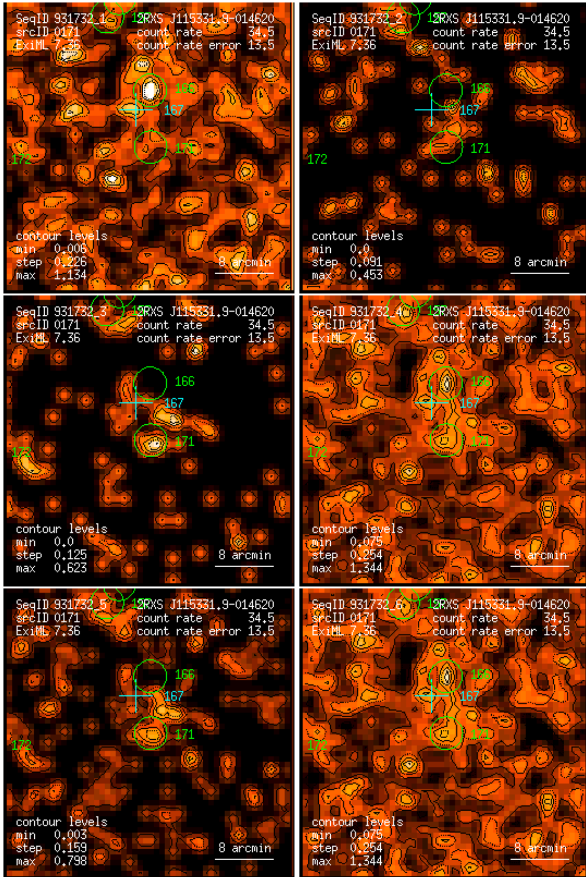
Figure 171: RASS 931732: detection 0171: band rate images, Gaussian filter: (1) PSPC channels 11 – 41, (2) 52 – 90, (3) 91 – 201, (4) 11 – 235, (5) 52 – 201, (6) 11 – 201. Broad band rates in counts/ks. Band rate contour levels in counts/ks/arcmin 2 .
