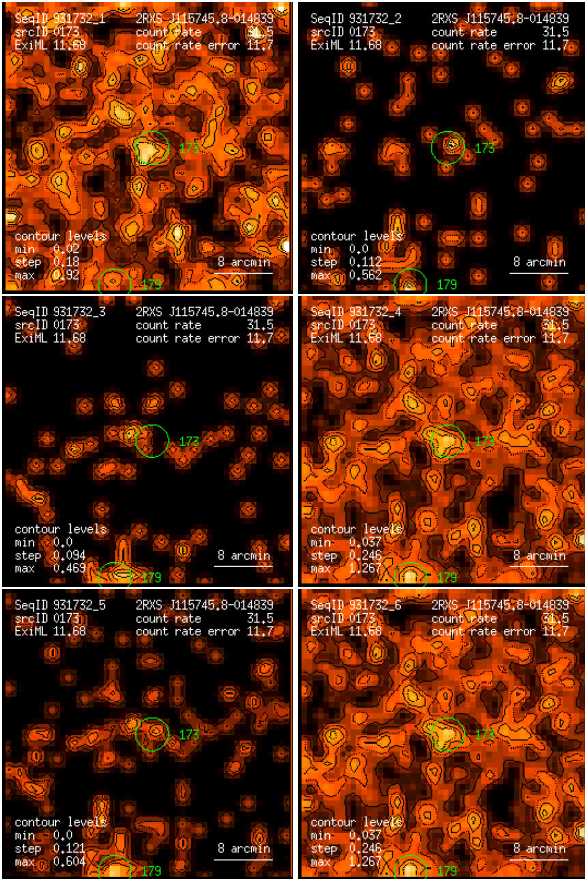
Figure 173: RASS 931732: detection 0173: band rate images, Gaussian filter: (1) PSPC channels 11 – 41, (2) 52 – 90, (3) 91 – 201, (4) 11 – 235, (5) 52 – 201, (6) 11 – 201. Broad band rates in counts/ks. Band rate contour levels in counts/ks/arcmin 2 .
