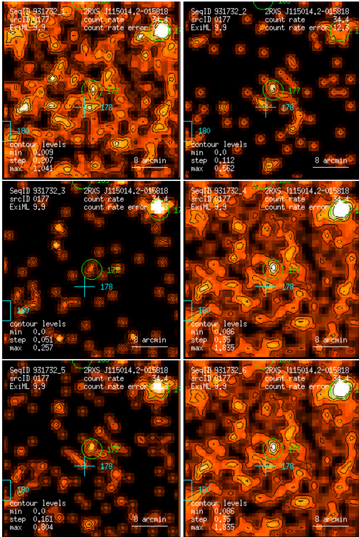
Figure 177: RASS 931732: detection 0177: band rate images, Gaussian filter: (1) PSPC channels 11 – 41, (2) 52 – 90, (3) 91 – 201, (4) 11 – 235, (5) 52 – 201, (6) 11 – 201. Broad band rates in counts/ks. Band rate contour levels in counts/ks/arcmin 2 .
