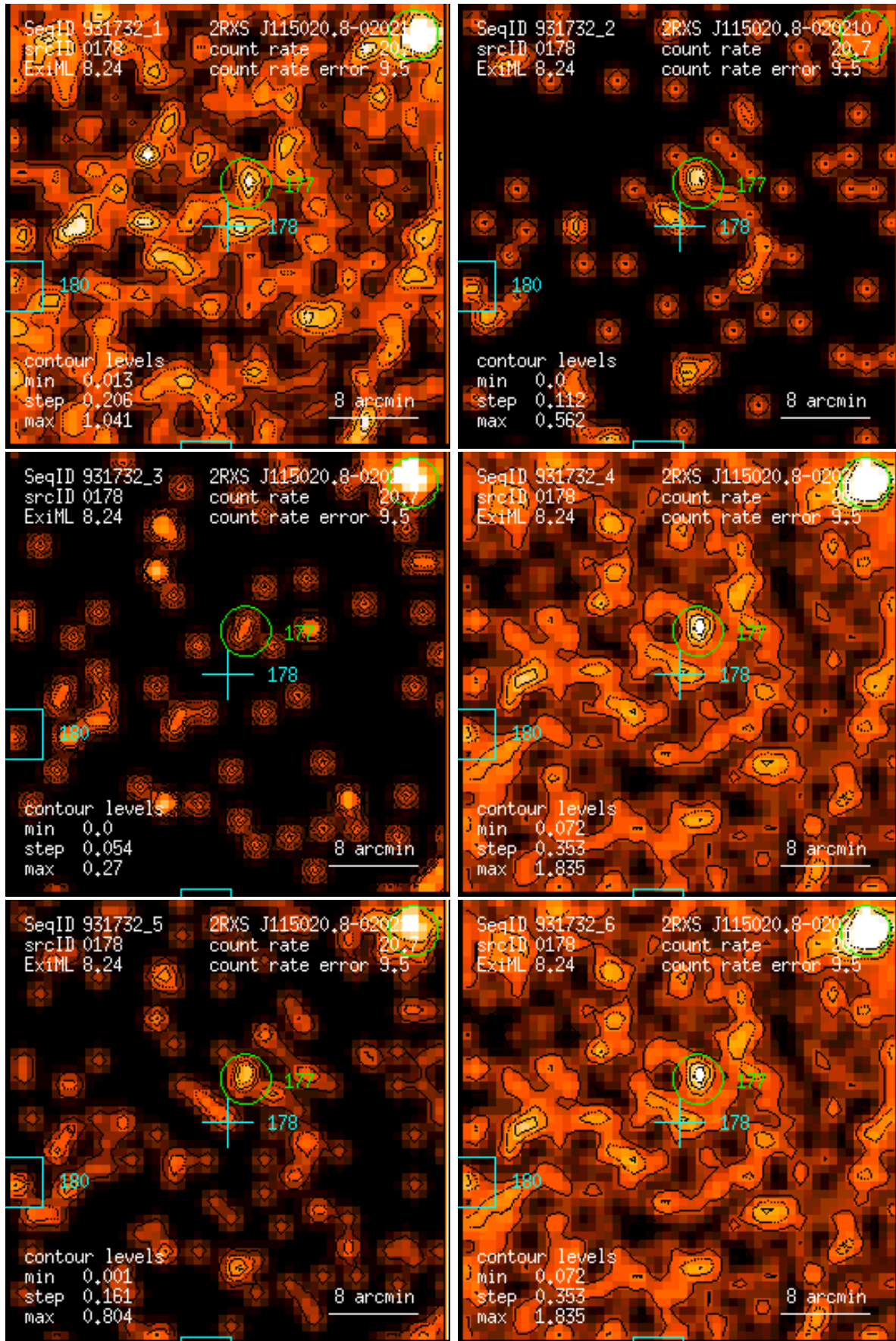
Figure 178: RASS 931732: detection 0178: band rate images, Gaussian filter: (1) PSPC channels 11 – 41, (2) 52 – 90, (3) 91 – 201, (4) 11 – 235, (5) 52 – 201, (6) 11 – 201. Broad band rates in counts/ks. Band rate contour levels in counts/ks/arcmin 2 .
