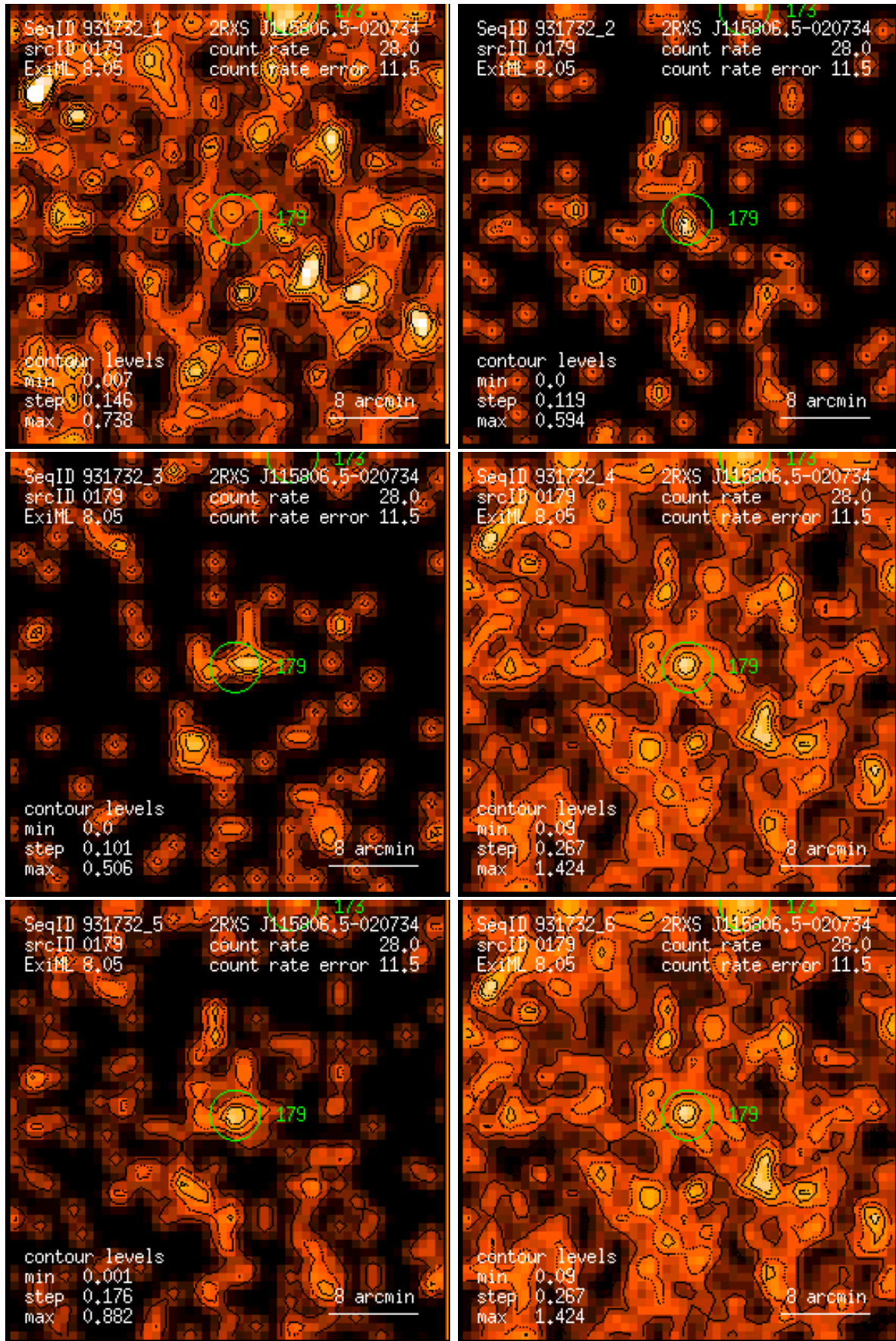
Figure 179: RASS 931732: detection 0179: band rate images, Gaussian filter: (1) PSPC channels 11 – 41, (2) 52 – 90, (3) 91 – 201, (4) 11 – 235, (5) 52 – 201, (6) 11 – 201. Broad band rates in counts/ks. Band rate contour levels in counts/ks/arcmin 2 .
