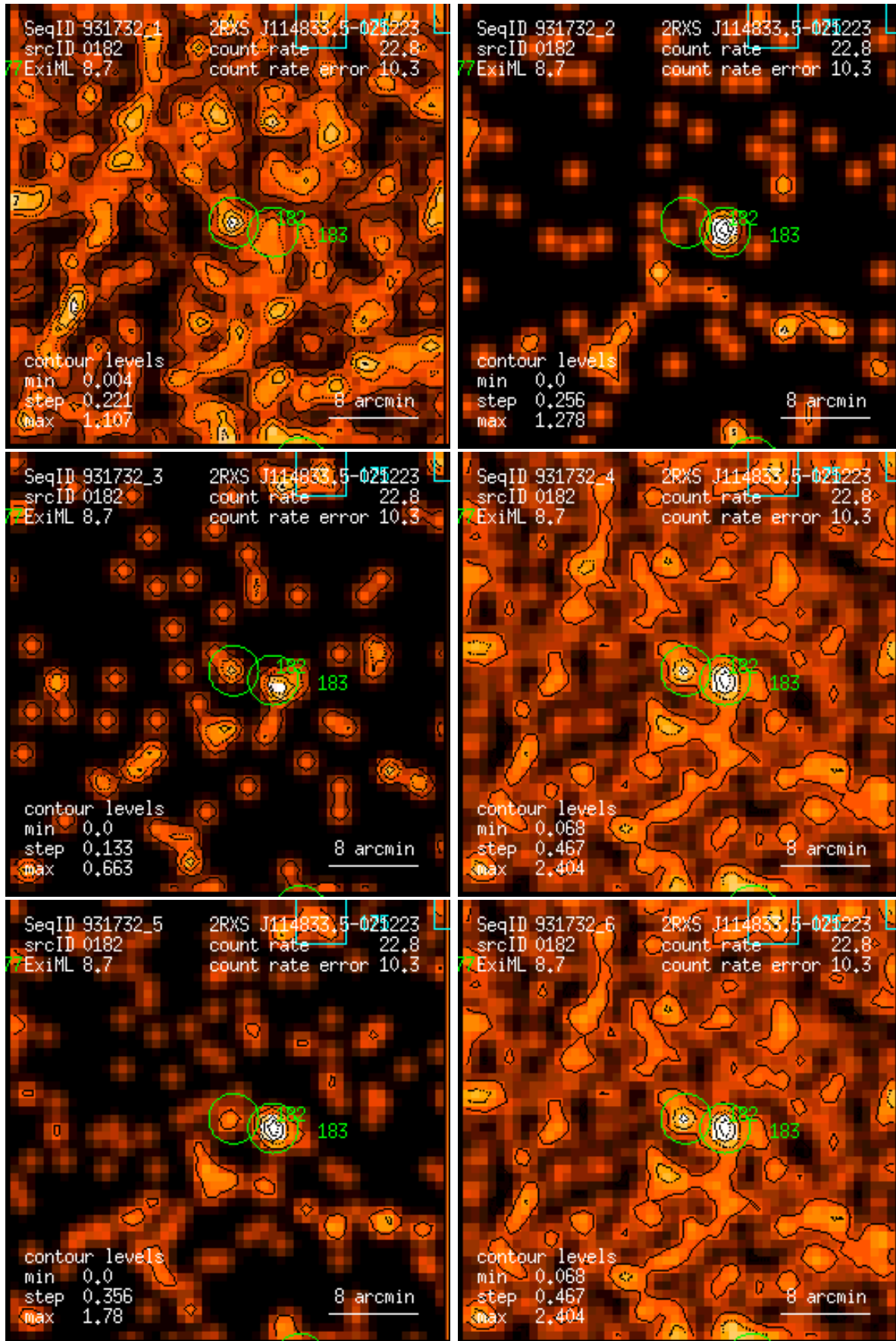
Figure 182: RASS 931732: detection 0182: band rate images, Gaussian filter: (1) PSPC channels 11 – 41, (2) 52 – 90, (3) 91 – 201, (4) 11 – 235, (5) 52 – 201, (6) 11 – 201. Broad band rates in counts/ks. Band rate contour levels in counts/ks/arcmin 2 .
