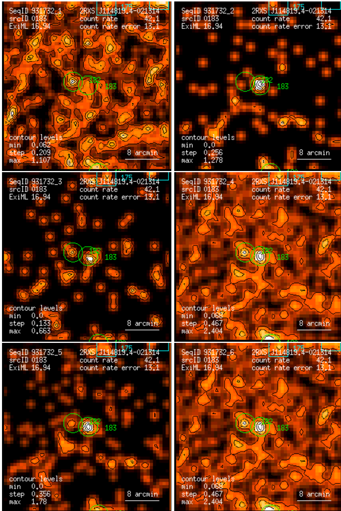
Figure 183: RASS 931732: detection 0183: band rate images, Gaussian filter: (1) PSPC channels 11 – 41, (2) 52 – 90, (3) 91 – 201, (4) 11 – 235, (5) 52 – 201, (6) 11 – 201. Broad band rates in counts/ks. Band rate contour levels in counts/ks/arcmin 2 .
