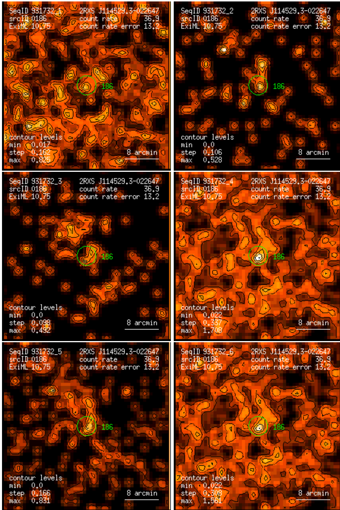
Figure 186: RASS 931732: detection 0186: band rate images, Gaussian filter: (1) PSPC channels 11 – 41, (2) 52 – 90, (3) 91 – 201, (4) 11 – 235, (5) 52 – 201, (6) 11 – 201. Broad band rates in counts/ks. Band rate contour levels in counts/ks/arcmin 2 .
