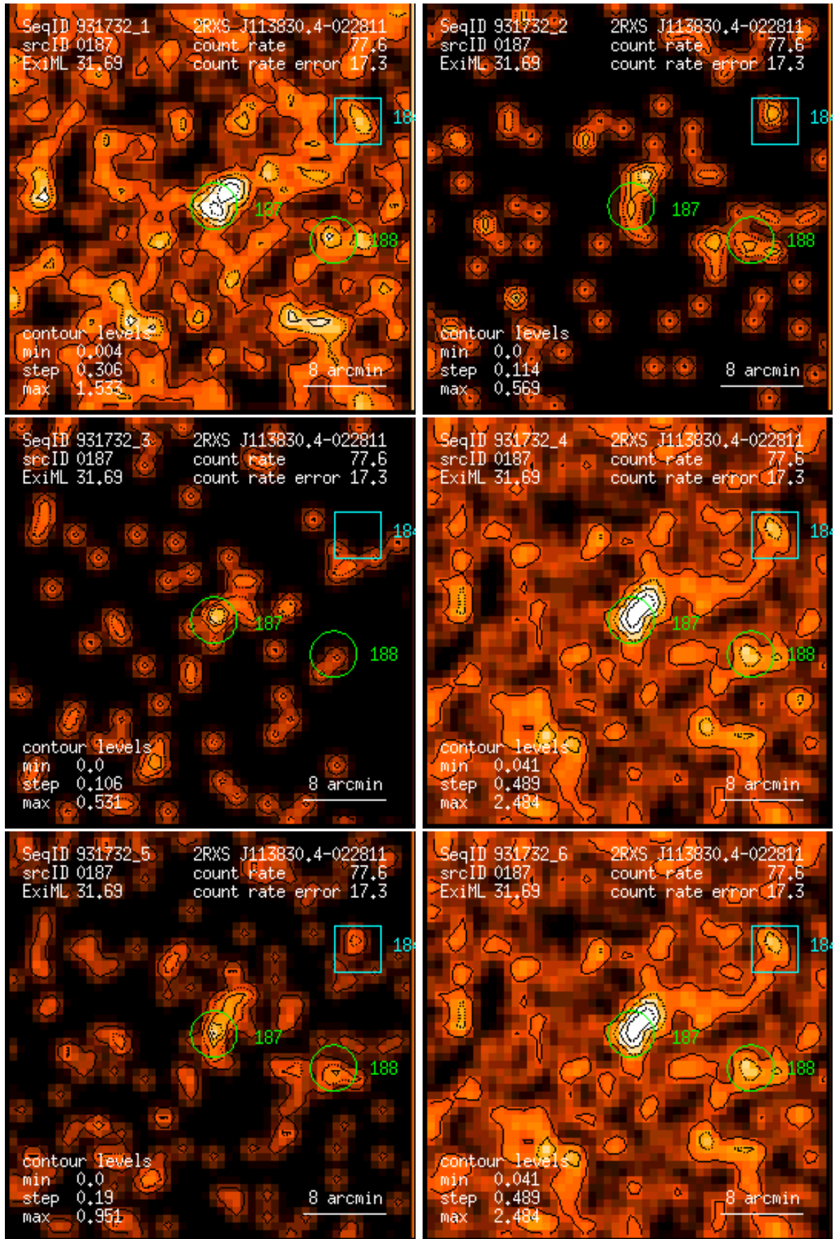
Figure 187: RASS 931732: detection 0187: band rate images, Gaussian filter: (1) PSPC channels 11 – 41, (2) 52 – 90, (3) 91 – 201, (4) 11 – 235, (5) 52 – 201, (6) 11 – 201. Broad band rates in counts/ks. Band rate contour levels in counts/ks/arcmin 2 .
