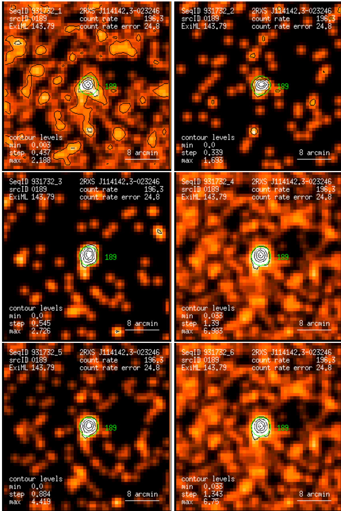
Figure 189: RASS 931732: detection 0189: band rate images, Gaussian filter: (1) PSPC channels 11 – 41, (2) 52 – 90, (3) 91 – 201, (4) 11 – 235, (5) 52 – 201, (6) 11 – 201. Broad band rates in counts/ks. Band rate contour levels in counts/ks/arcmin 2 .
