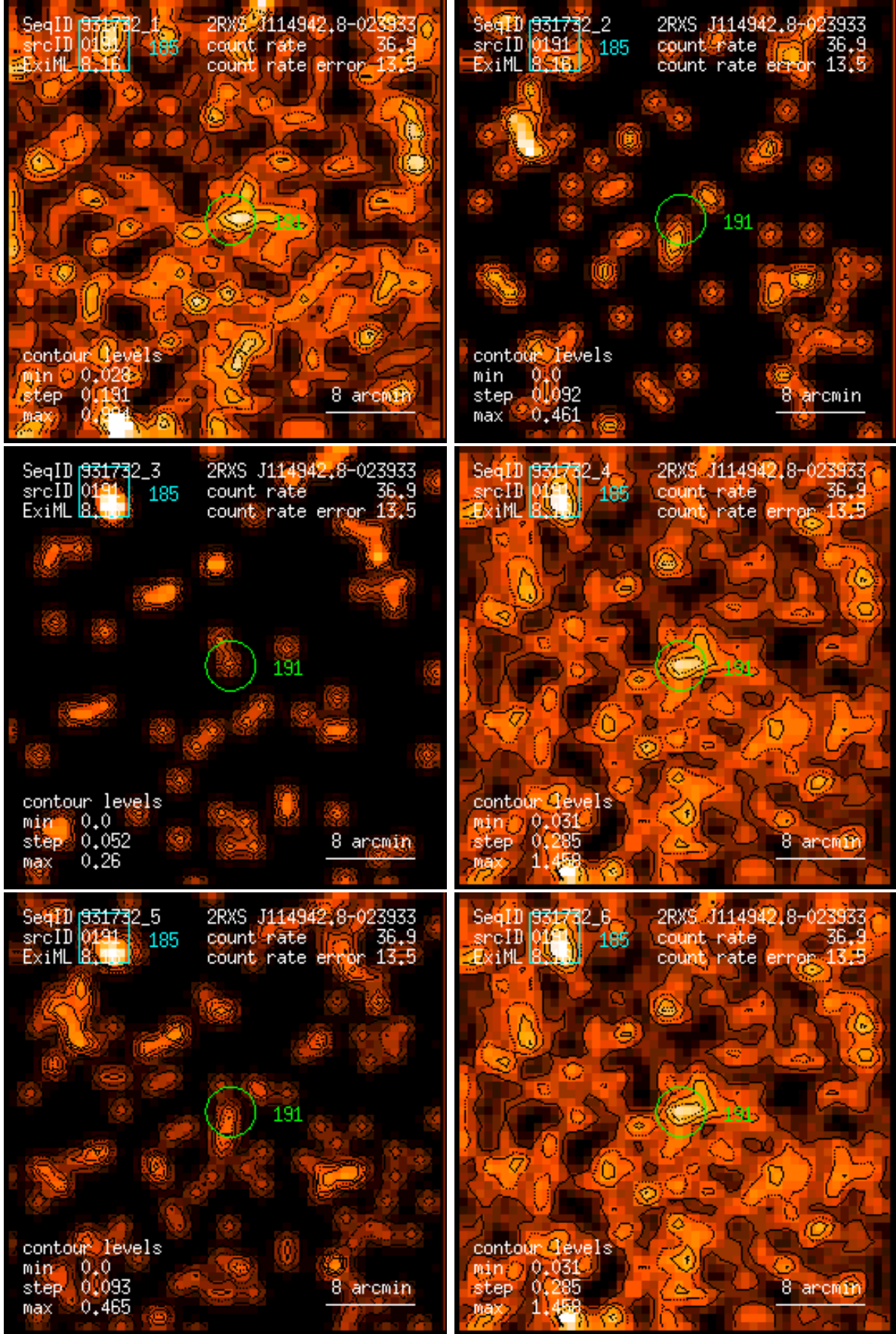
Figure 191: RASS 931732: detection 0191: band rate images, Gaussian filter: (1) PSPC channels 11 – 41, (2) 52 – 90, (3) 91 – 201, (4) 11 – 235, (5) 52 – 201, (6) 11 – 201. Broad band rates in counts/ks. Band rate contour levels in counts/ks/arcmin 2 .
