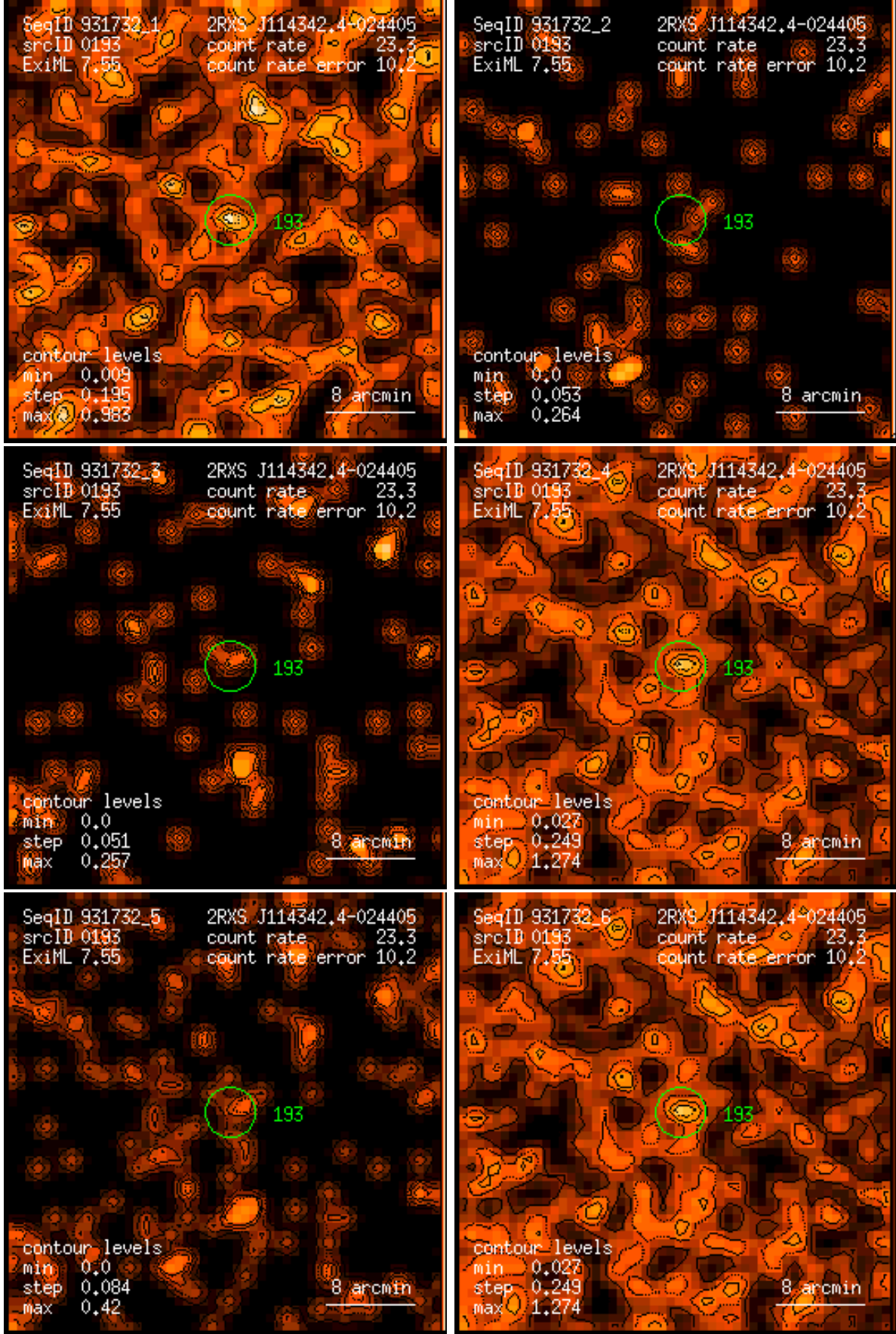
Figure 193: RASS 931732: detection 0193: band rate images, Gaussian filter: (1) PSPC channels 11 – 41, (2) 52 – 90, (3) 91 – 201, (4) 11 – 235, (5) 52 – 201, (6) 11 – 201. Broad band rates in counts/ks. Band rate contour levels in counts/ks/arcmin 2 .
