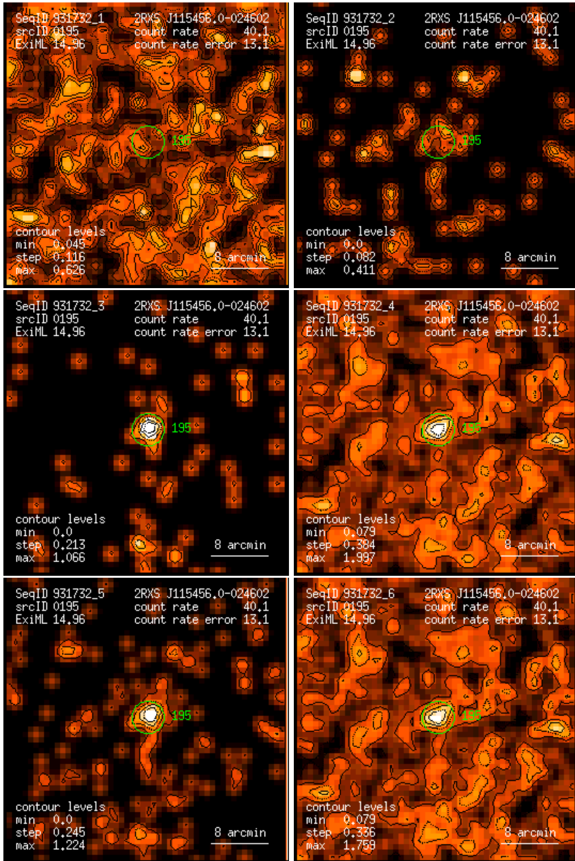
Figure 195: RASS 931732: detection 0195: band rate images, Gaussian filter: (1) PSPC channels 11 – 41, (2) 52 – 90, (3) 91 – 201, (4) 11 – 235, (5) 52 – 201, (6) 11 – 201. Broad band rates in counts/ks. Band rate contour levels in counts/ks/arcmin 2 .
