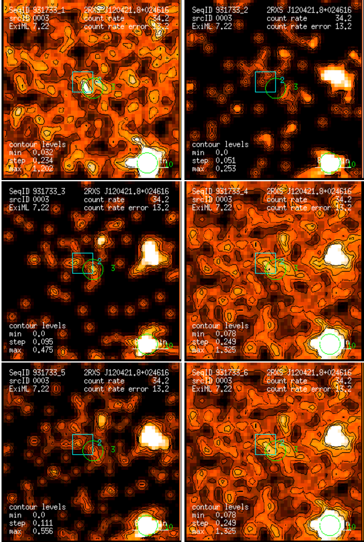
Figure 3: RASS 931733: detection 0003: band rate images, Gaussian filter: (1) PSPC channels 11 – 41, (2) 52 – 90, (3) 91 – 201, (4) 11 – 235, (5) 52 – 201, (6) 11 – 201. Broad band rates in counts/ks. Band rate contour levels in counts/ks/arcmin 2 .
